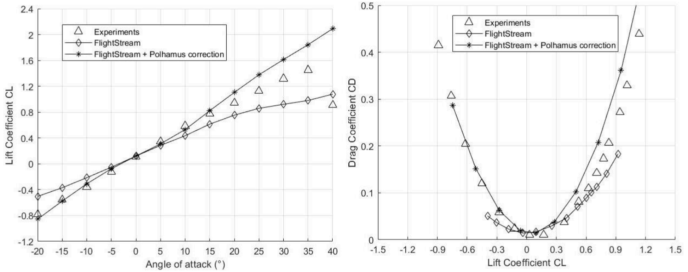
Fig. 16 Lift and Drag Polar for a subsonic flow at V = 100 \text{ ft/sec} and at Re_{mac} = 0.33 \times 10^6 for a 60^\circ swept delta wing.
