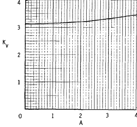
Fig. 6 Variation of K_v with AR for delta wings [18].
