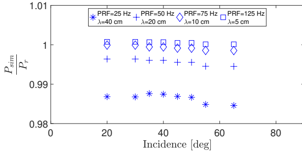
Fig. 4: \frac{P_{sim}}{P_r} , difference from 1 are assumed to be due to (a) power outside the integration domain (b) numerical rounding, 2 nd of August, \psi = 0^\circ , v_y = 10 m/s.
