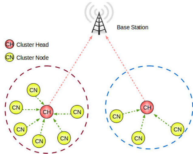
Fig. 1. Clustering model
