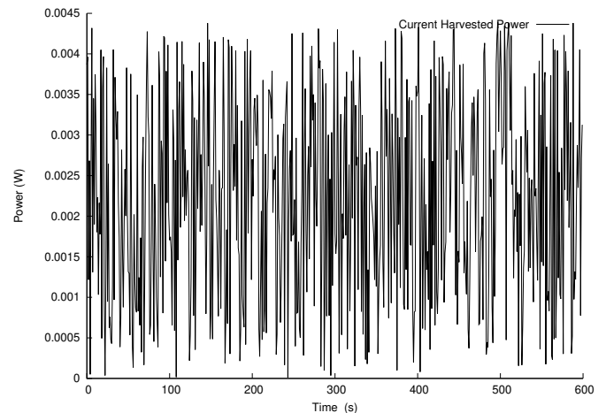
Fig. 2. Current PEG harvested energy
