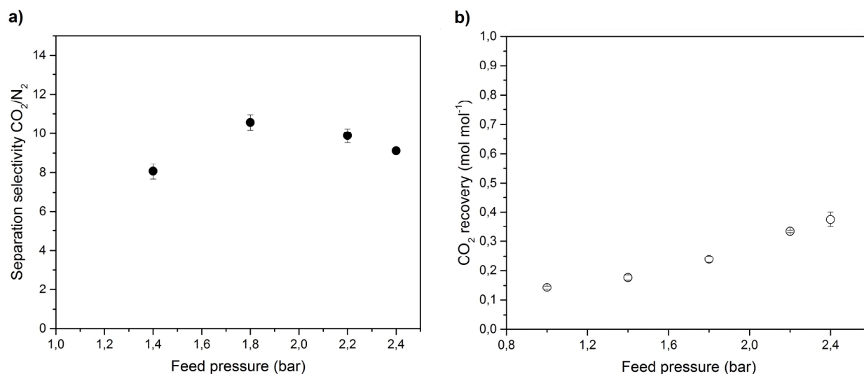
Fig. 6. Separation selectivities (6-a) for \text{CO}_2/\text{N}_2 mixture and \text{CO}_2 recovery (6-b) at different pressures (Temperature = 21°C, sweep/feed ratio = 1, flowrate of feed = 10 L/min, \text{CO}_2 concentration in the feed stream = 10%, and using pure \text{N}_2 as the sweep gas)
