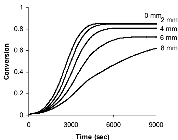
Fig.9. Degree-of-cure distribution during the cure
