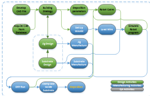
Figure 16 - Design for AM
