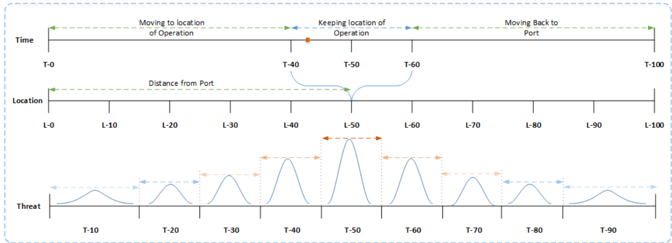
Figure 12 - Factors
