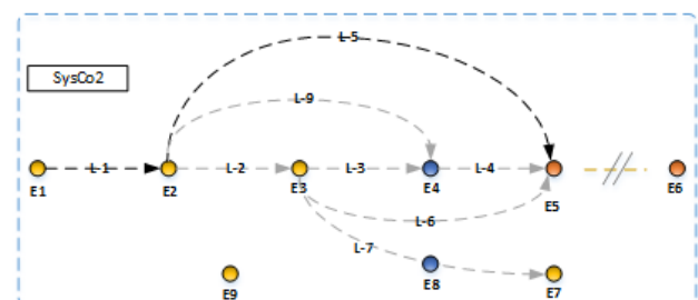
Figure 5 - SysCo2
