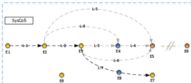
Figure 8 - SysCo5
