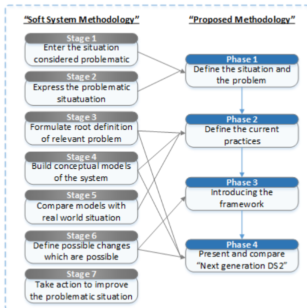
Figure 1 - Research Methodology
