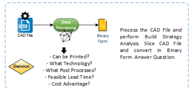
Figure 18 - AM assessment
