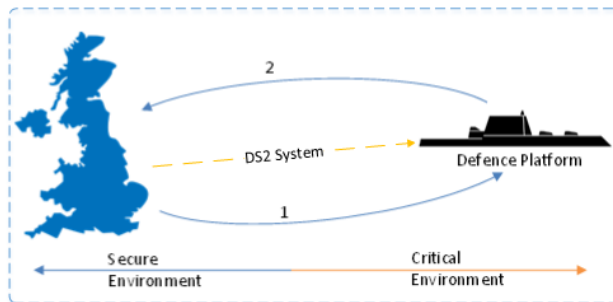
Figure 13 - Mission Loop
