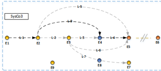
Figure 6 - SysCo3
