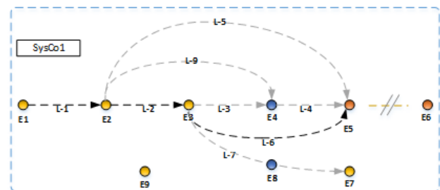
Figure 4 - SysCo1
