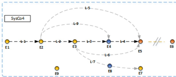
Figure 7 - SysCo4
