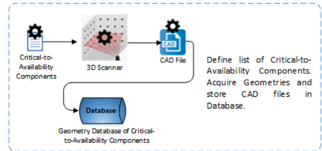
Figure 17 - Geometries database
