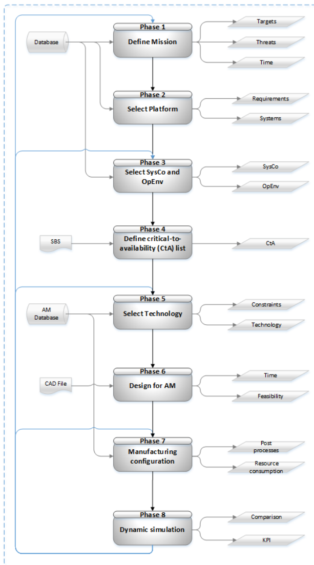
Figure 20 - Framework
