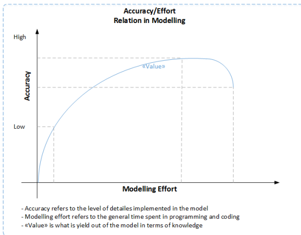
Figure 3 - Accuracy/Effort relation
