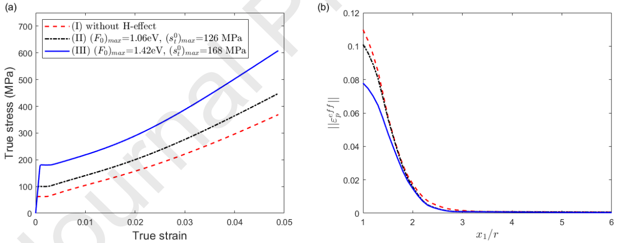
Fig. 12. (a) True tensile stress-strain curves with different activation energy F_0 and thermal slip resistance s_t^0 , leading to various H-enhanced yield strength. These curves are obtained using the DSS-CP model for Ni single crystals, loaded in uniaxial tension along the [100] direction. Cases (II) and (III) correspond to the H-affected stress-strain curves with extremely high uniform H concentration (i.e., C_L/C_0=1 throughout the field). (b) Effective plastic strain as a function of the normalized radial distance along the crack direction for the two-way coupled problem.
