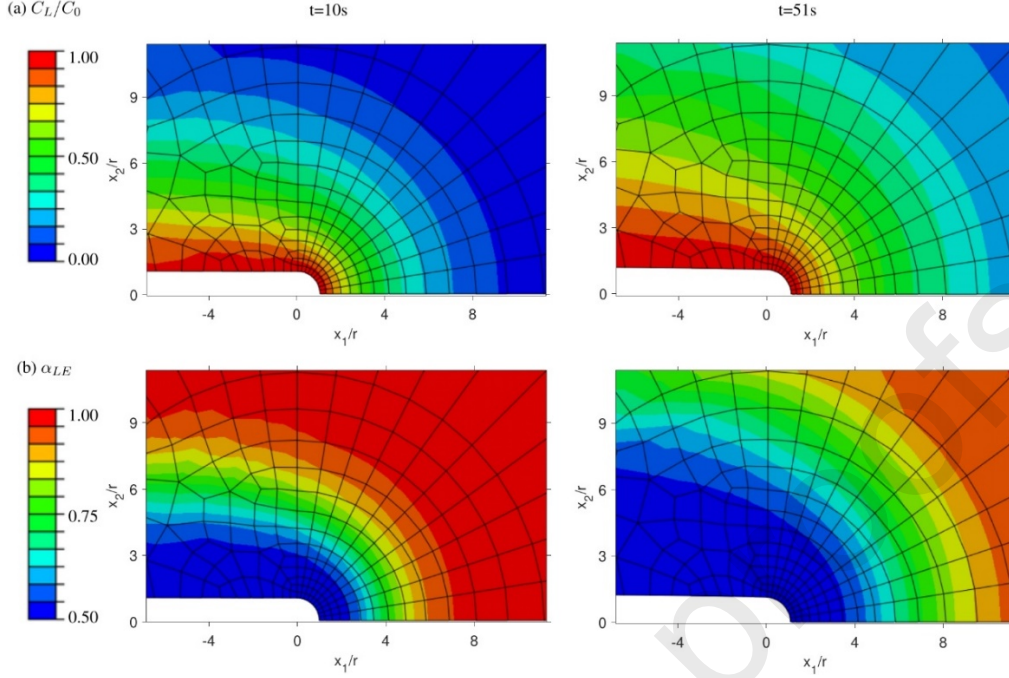
Fig. 5. Contours of (a) normalized H lattice concentration C_L/C_0 and (b) line tension coefficient \alpha_{LE} at t=10 s (left column) and 51 s (right column), near the notch root. The far-field monotonic loading is applied throughout this work, with K_I = 10 \text{ MPa}\sqrt{m} , applied over a total rise time of 51s. The local value of \alpha_{LE} at each integration point is updated based on the local value of C_L . The notch radius is denoted by r .
