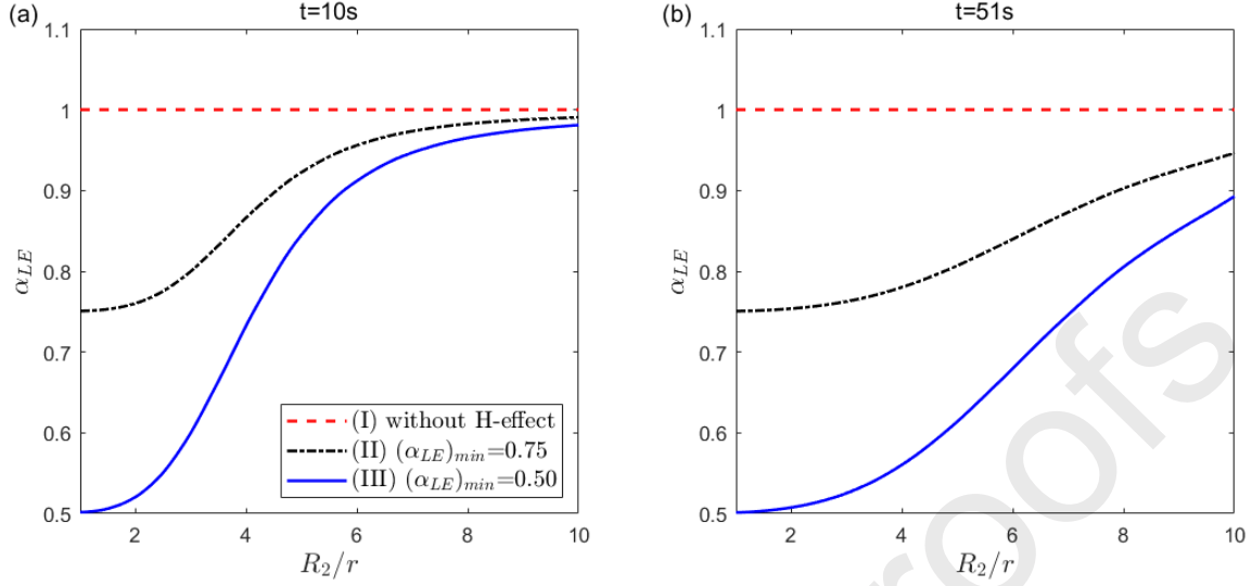
Fig. 10. Evolution of the line tension coefficient \alpha_{LE} as a function of the normalized radial distance along the slip line direction R_2/r : (a) at t=10s ; (b) at t=51s for the cases (I) without H effect, i.e., \alpha_{LE}=1.0 throughout the simulation, (II) (\alpha_{LE})_{min}=0.75 , and (III) (\alpha_{LE})_{min}=0.50 at the notch root. Here, R_2 is an example which pertains to the conjugate pair of slip systems (\bar{1}11)[101] & (11\bar{1})[101] ; Profile of (\alpha_{LE})_{min} along R_1/r and R_3/r display a similar trend. The \alpha_{LE} is updated based on the C_L distribution.
