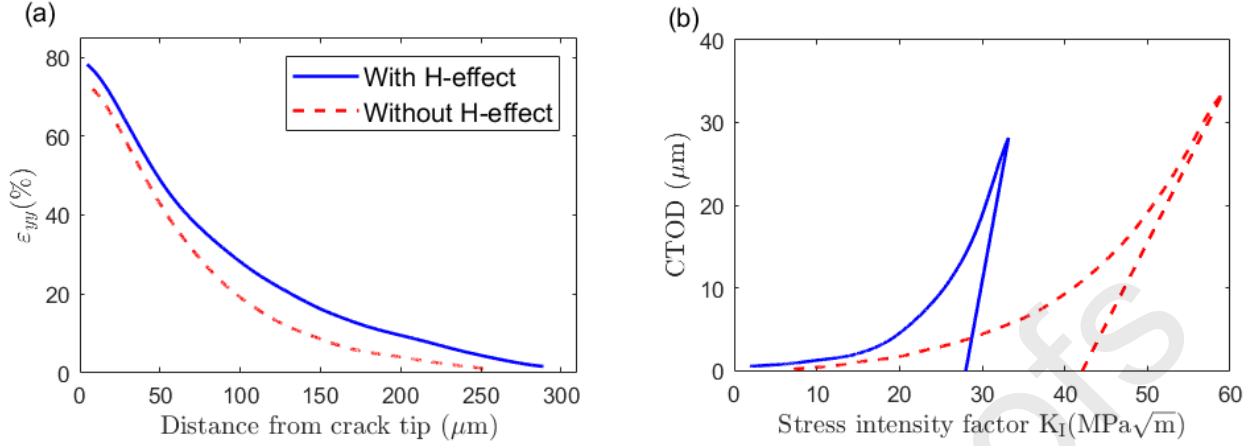
Fig. 15. Available experimental data for the validation of the trend of model prediction (Sun et al., 1995): (a) H-effect on the tensile strain parallel to the crack axis direction (i.e., \varepsilon_{yy} ) as a function of the radial distance in advance of the crack. The corresponding max stress intensity is K_I = 35.00 \text{ MPa}\sqrt{\text{m}} ; (b) CTOD as function of the stress intensity ( K_I ).
