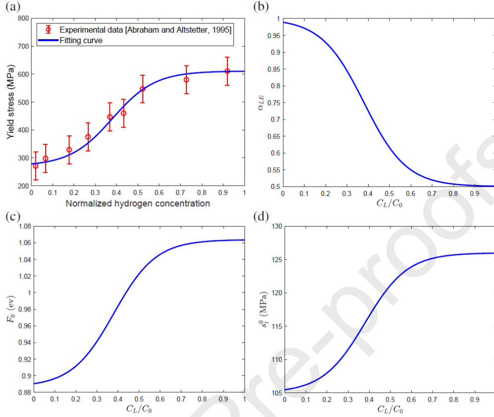
Fig. 3. (a) Experimental yield strength (Abraham and Altstetter, 1995) and its sigmoidal interpolation. Assumed dependence of DSS-CP parameters on the normalized H concentration C_L/C_0 for (b) line tension coefficient \alpha_{LE} , (c) activation energy F_0 , and (d) thermal slip resistance s_t^0 . The sigmoidal relations in (b)-(d) are determined by the interpolation in (a).
