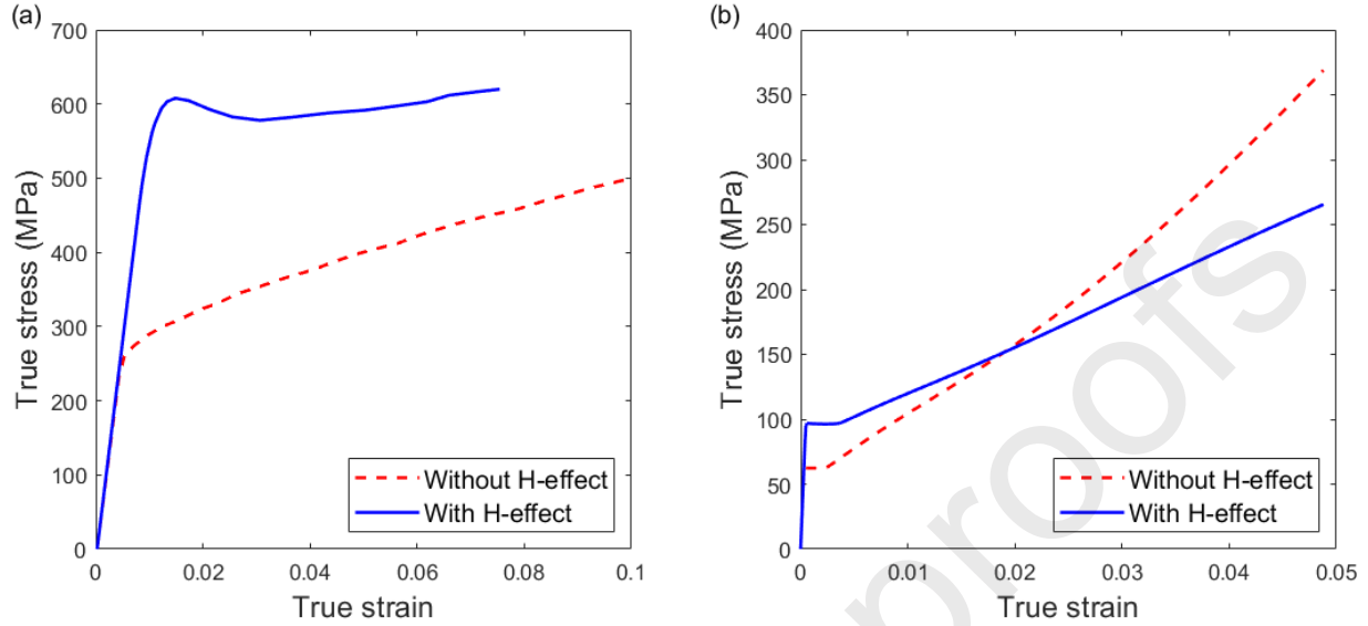
Fig. 2. (a) Experimental stress-strain curves for polycrystalline FCC 310 SS without and with H charged (Abraham and Altstetter, 1995). The experiments demonstrate that with a near-saturated high H concentration, the yield strength is doubled, while the strain hardening rate is reduced by half for common FCC metals. (b) Bounds on H effects on uniaxial tensile true stress-strain curves simulated by the H-dependent DSS-CP model (Castelluccio et al., 2018) for Ni single crystals loaded along the [010] direction at a strain rate of 10^{-3} \text{ s}^{-1} at room temperature. Refer to Appendix C for calibration of the DSS-CP parameters without H. Model responses with extremely high uniform H concentration (i.e., C_L/C_0=1 ) and without H are compared. The activation energy F_0 and thermal slip resistance S_t^0 depend on H concentration, accounting for H-doubled yield strength. Simultaneously, the line tension coefficient \alpha_{LE} accounts for the reduced strain hardening rate by half with H.
