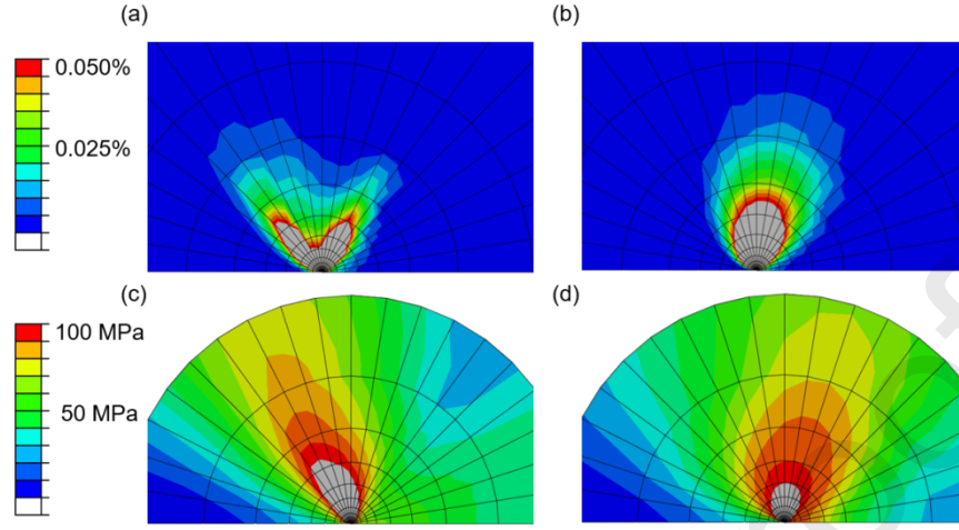
Fig. 18. Comparison between DSS-CP and J_2 plasticity models: (a)-(b) effective plastic strain field obtained by DSS-CP and J_2 plasticity, respectively; (c)-(d) von Mises stress field obtained by DSS-CP and J_2 plasticity, respectively.
