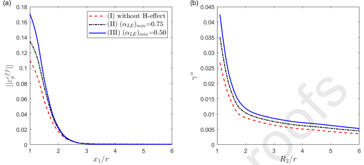
Fig. 11. (a) Effective plastic strain as a function of the normalized distance ahead of the crack front for different cases of \alpha_{LE} profiles, i.e., (I) without H-effect, (II) (\alpha_{LE})_{min}=0.75 and (III) (\alpha_{LE})_{min}=0.50 ; (b) Plastic shear strain \gamma^\alpha pertain to the conjugate pair of slip system (\bar{1}11)[101] & (11\bar{1})[101] as a function of its normalized radial distance along the slip line direction R_2/r . A greater degree of reduction of the strain hardening rate with H leads to more significant enhancement of crack tip plasticity. The initial boundary value has been outlined in Section 4 with t = 51 s rise time to a peak loading condition of K_I = 10 \text{ MPa}\sqrt{m} which are applied to all the other simulations throughout the work.
