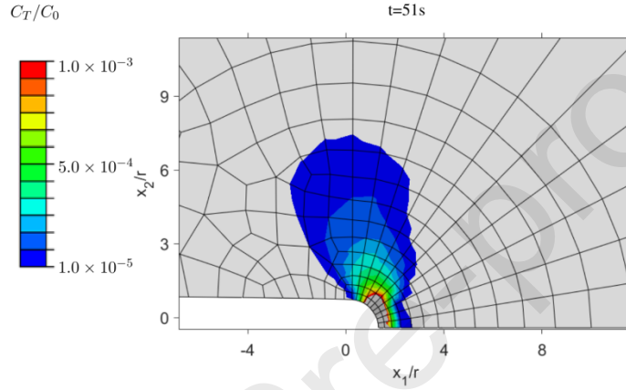
Fig. 6. Contours of normalized H trap concentration C_T/C_0 at t=51\text{s} . The gray regions near the crack tip indicate C_T/C_0 values greater than 10^{-3} , whereas the gray regions distant from the crack tip represent C_T nearly equal to 0.
