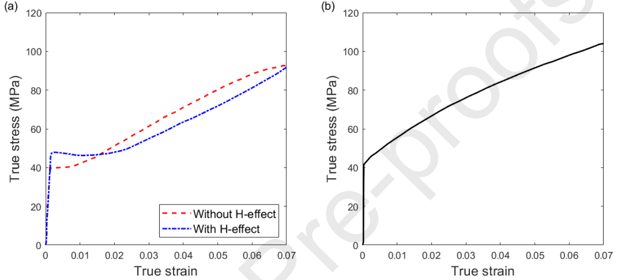
Fig. 16. (a) Monotonic stress-strain curves with and without H charged for single crystal FCC Ni, oriented along [167] at a strain rate of 9 \times 10^{-5} \text{ s}^{-1} (Yagodzinsky et al., 2009). (b) Model responses of DSS-CP without H-effect for single crystal Ni (Castelluccio and McDowell, 2017). Experimental data demonstrates H-enhanced yield strength, as well as H-induced reduction of the strain hardening rate.
