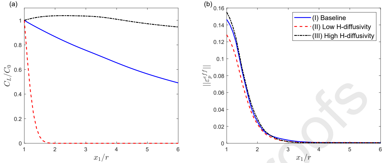
Fig. 13. (a) Normalized H-concentration as a function of the normalized distance ahead of the crack front with various H-diffusivity D assigned. For the two-way coupled problem, the same initial boundary value has been used in Section 4 with t = 51 s rise time to a peak loading condition of K_I = 10 \text{ MPa}\sqrt{m} . (b) Effective plastic strain as a function of the normalized distance ahead of the crack front. Higher H-diffusivity leads to more significant enhancement of the near crack tip plasticity.
