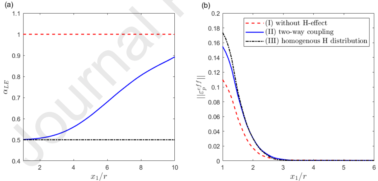
Fig. 14. (a) Line tension coefficient \alpha_{LE} as a function of x_1/r at t=51\text{s} for the three cases: (I) without H-effect, i.e., \alpha_{LE} remains constant at 1.0; (II) two-way coupling algorithm, i.e., \alpha_{LE} updated based on the evolution of C_L ; (III) homogenous H-distribution assumption resulting in a constant \alpha_{LE} of 0.5 throughout simulation. (b) Model responses of the effective plastic strain in terms of x_1/r for these three cases.
