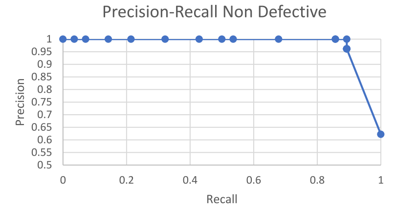
Fig. 16. Precision-Recall curve for non-defective annotations.
