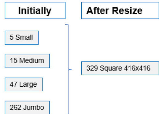
Fig. 9. Image resizing.
