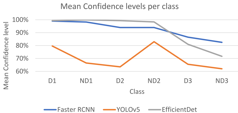
Fig. 22. Mean threshold per model.
