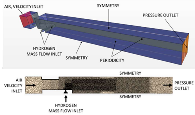
FIGURE 5: FLUID REGION OF A SINGLE INJECTOR WITH BOUNDARY DEFINITIONS (TOP) AND MESH (BOTTOM)
