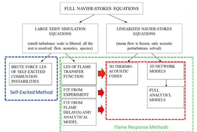
FIGURE 4: APPROACHES TO THERMOACOUSTIC ANALYSIS (AFTER [13])
