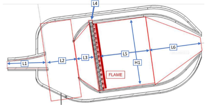
FIGURE 14: COMBUSTOR GEOMETRY SHOWING DIMENSIONS VARIED IN THE SENSITIVITY ANALYSIS
