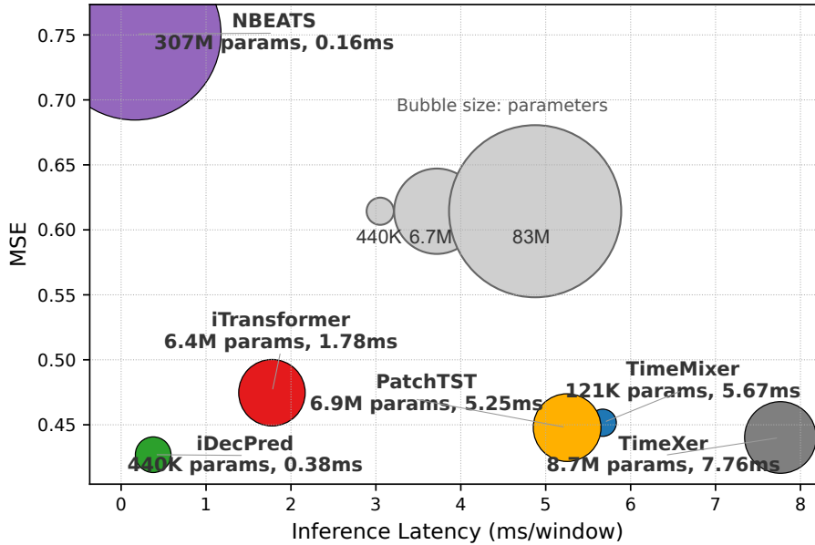
Figure 4.6: Efficiency–accuracy trade-offs on the C_862 dataset ( L=96, H=96 ). Bubble size denotes parameter count.
