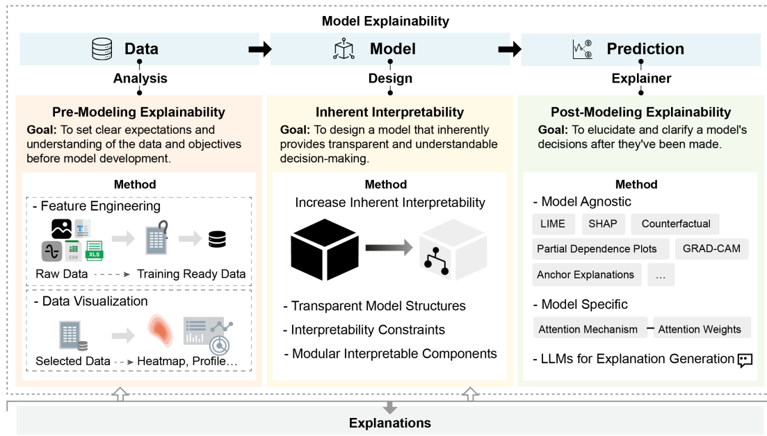
Figure B.4: A Comprehensive Framework for Model Explainability in Machine Learning.
