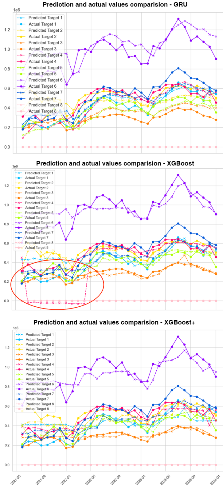
Figure 3.2: Comparison of GRU, XGBoost, and XGBoost+ predictions against ground truth for boarding areas A–G and Other (targets 1–8).
