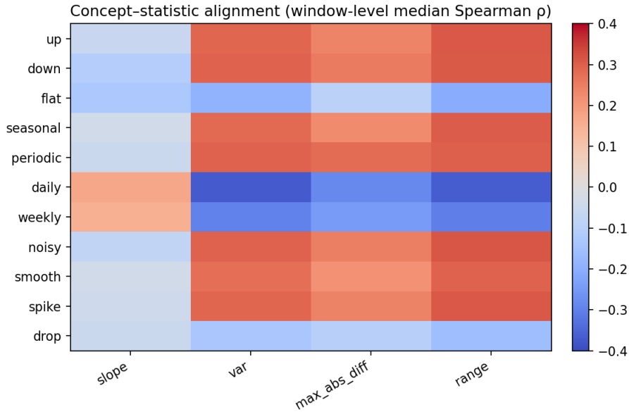
Figure 5.7: Concept-score anchoring to patch statistics (median Spearman \rho heatmap)
