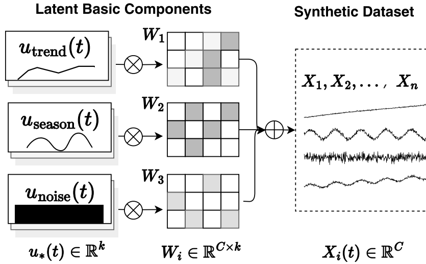
Figure 4.3: Synthetic Data Generation Pipeline. Latent trend/seasonal/noise bases are projected by W_k and summed to form X(t) . Optional local, causal, and calendar effects as well as anomalies and missingness can be injected to increase difficulty.
