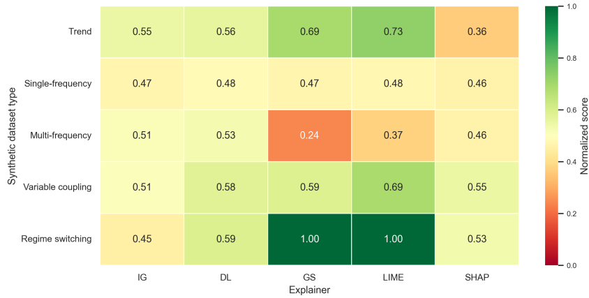
Figure 2.2: Oracle-score heatmap on synthetic datasets using the regenerated analysis output (all seeds), following the unified normalization protocol defined in Section 2.5.
