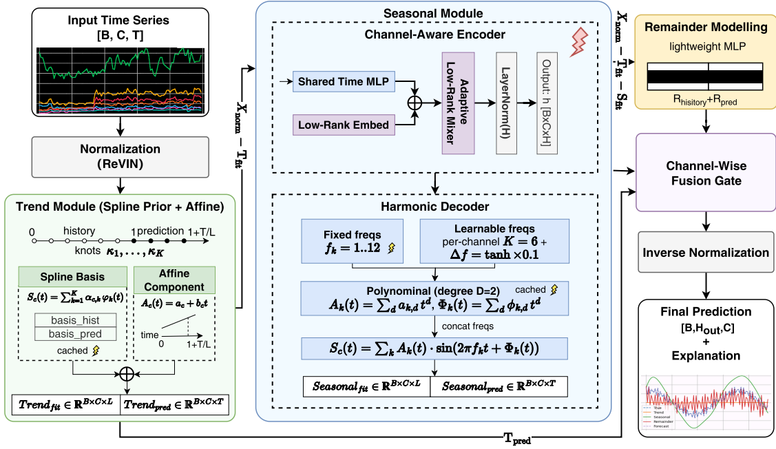
Figure 4.1: Overall architecture of iDecPred. The model normalises inputs with Reversible Instance Normalisation (ReVIN), decomposes them into trend (spline + affine), seasonal (channel-aware encoder with harmonic decoder), and residual (Multi-Layer Perceptron (MLP)) components, and fuses their forecasts via a channel-wise attention gate to produce final predictions with interpretable components.
