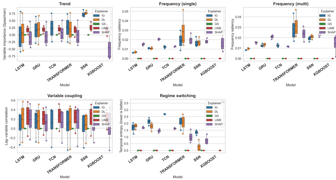
Figure 2.5: Cross-seed variability of synthetic oracle metrics (seeds 42–44). Panels correspond to the five synthetic dataset types and use each dataset’s primary oracle metric. Within each panel, models are on the x-axis, explainers are colour-coded, and each box summarises three seed values for one model–explainer pair (with jittered seed points).
