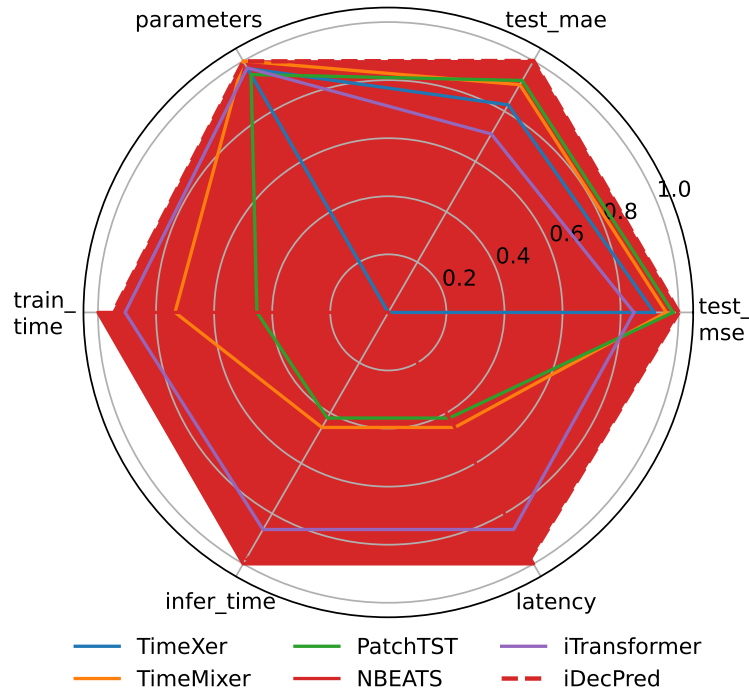
Figure 4.5: Average radar chart of forecasting performance across 16 synthetic datasets under the 96–96 setting. Curves closer to the boundary indicate better performance.
