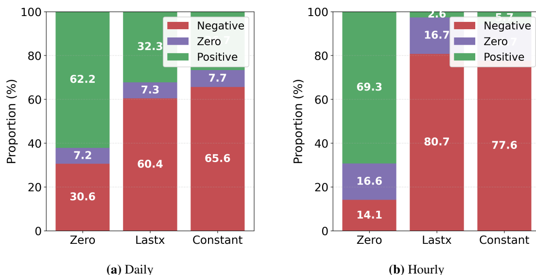
Figure 5.9: Delta sign proportions for daily and hourly models on the test split. Each bar shows the proportion of forecast steps with negative, zero, and positive deltas under different scenarios (zero, lastx, constant).
