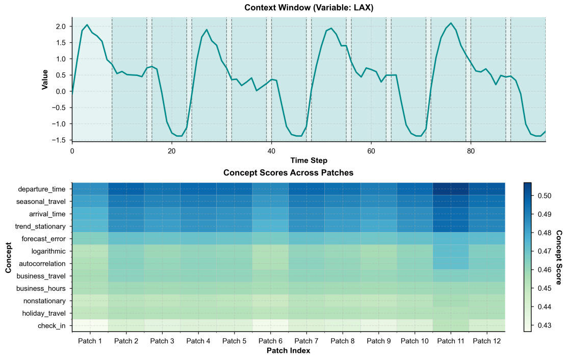
Figure 5.5: Concept-based explanations for one input window. Top: the selected context window (one variable) with patch boundaries. Bottom: heatmap of concept scores over patches; concepts are selected by highest activation in this window (max over patches).
