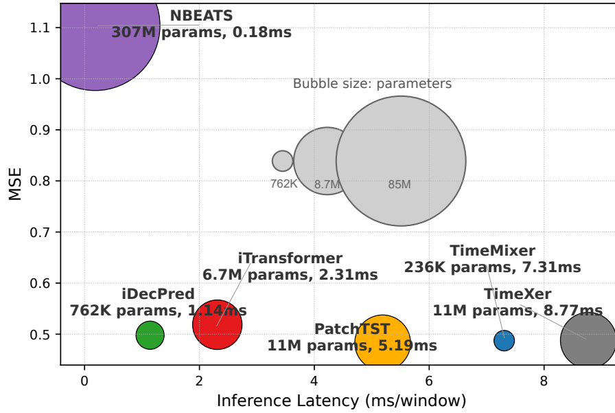
Figure 4.7: Efficiency–accuracy trade-offs on the C_862 dataset ( L=96, H=720 ). Bubble size denotes parameter count.
