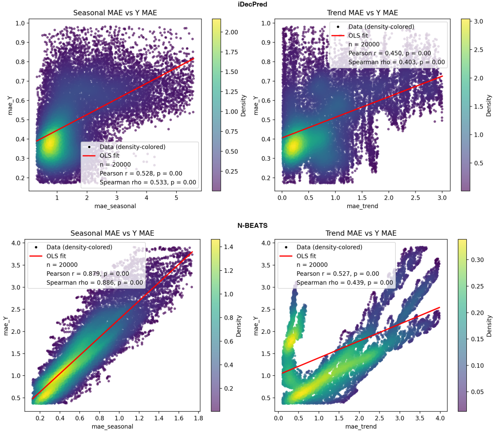
Figure 4.9: Decomposition–forecast relationship on C.7. Top row: iDecPred; bottom row: N-BEATS. (a) seasonal MAE vs. MAE Y (iDecPred); (b) trend MAE vs. MAE Y (iDecPred); (c) seasonal MAE vs. MAE Y (N-BEATS); (d) trend MAE vs. MAE Y (N-BEATS). Each point is a \langle \text{window}, \text{channel} \rangle ; color encodes local density; red line is an OLS fit. Legends report n , Pearson r , and Spearman \rho .
