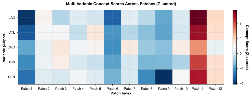
Figure 5.6: Multi-variable concept score heatmap at aligned patch indices. Rows are variables (airports) and columns are patch indices over the same context window; colors show the selected concept score across variables for each patch index (z-scored for visualisation).
