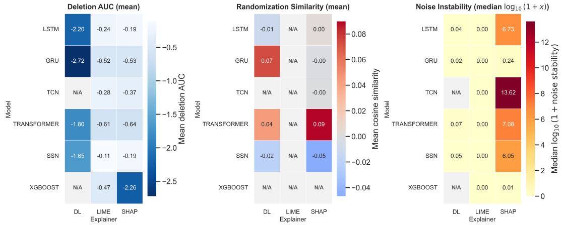
Figure 2.6: Overview of behavioural explainability metrics on real-world airport data, aggregated across the four representative datasets. Rows correspond to forecasting models and columns to explainers. Left: mean deletion AUC (more negative = larger performance degradation under deletion). Middle: mean model-randomisation similarity (cosine similarity between original and randomised-model attributions; values near zero indicate stronger sensitivity to learnt parameters). Right: median \log_{10}(1 + \text{noise stability}) under input perturbations. N/A indicates an inapplicable or undefined case: TCN–DeepLift is omitted for the same Captum limitation as in the synthetic benchmark; XGBoost randomisation is not defined in this pipeline; and some neural-model LIME randomisation entries are undefined due to degenerate randomised-model attribution vectors (NaN cosine similarity).
