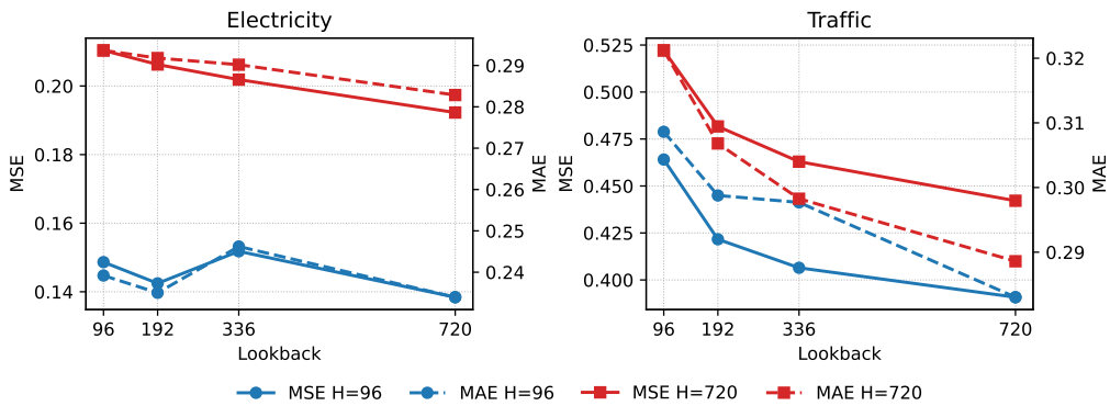
Figure 4.4: iDecPred performance on forecast horizons 96 and 720 with varying look-back lengths L \in \{96, 192, 336, 720\} on the Electricity and Traffic.
