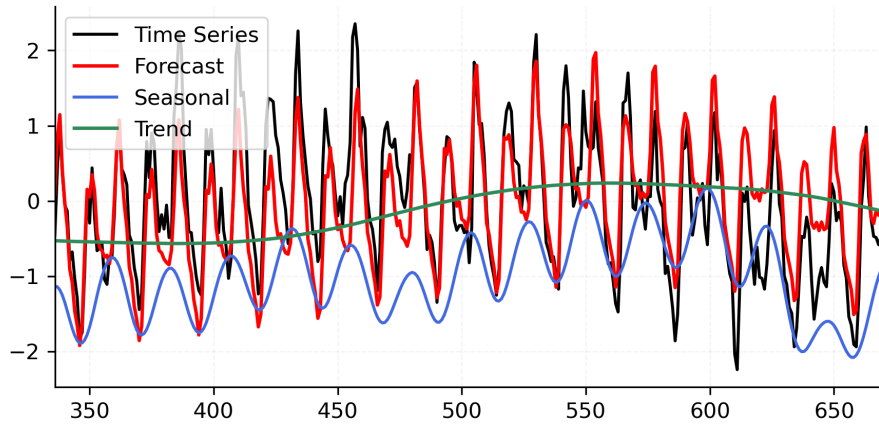
Figure 4.8: iDecPred decomposition on the Electricity dataset. The model jointly outputs trend, seasonal and final forecast components, enabling interpretable inspection on real-world data without access to ground-truth decompositions.
