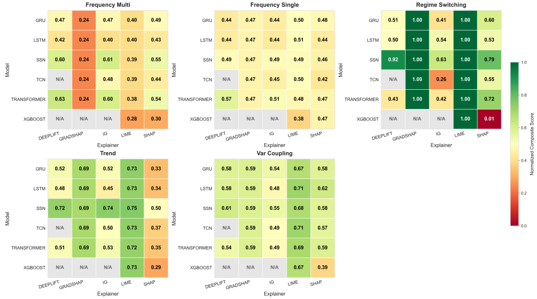
Figure 2.3: Model-explainer interaction heatmap on synthetic datasets, showing composite explainability scores across forecasting models and dataset types under the unified normalization protocol defined in Section 2.5.
