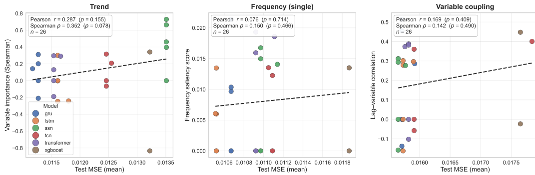
Figure 2.4: Aggregate relationship between prediction error (mean test MSE) and dataset-specific oracle metrics for seed 42. Each point is one model-explainer combination; each panel (trend, frequency-single, var-coupling) has n = 26 points.
