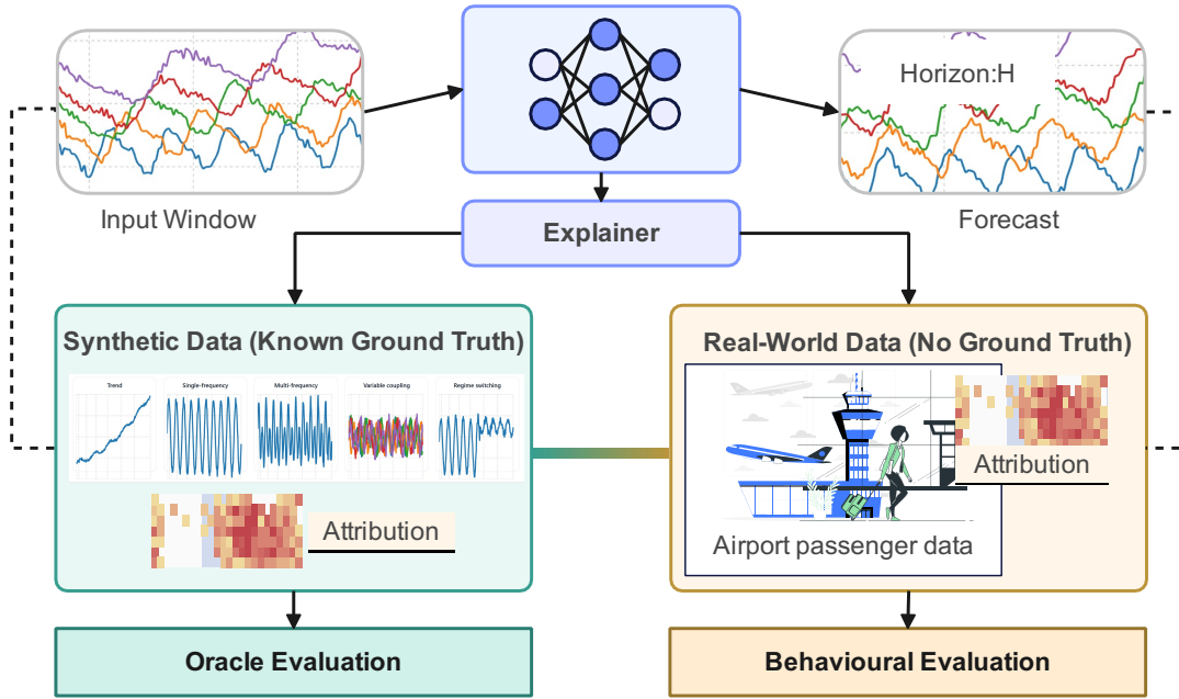
Figure 2.1: Dual evaluation framework for explainability. Synthetic datasets enable oracle-based evaluation against predefined attribution targets, while real-world datasets are assessed using behavioural metrics that probe model sensitivity and attribution robustness.
