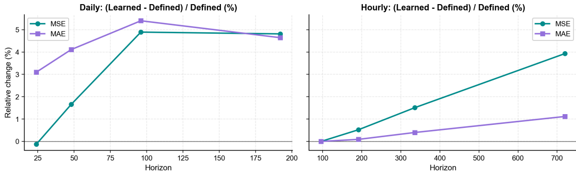
Figure 5.4: Concept ablation (relative MSE and MAE change vs defined concepts). Both MSE and MAE show the relative change when using learned concepts compared to defined concepts.
