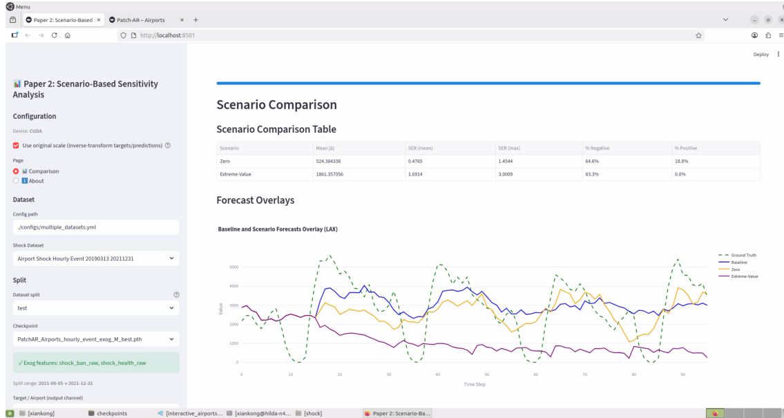
Figure 5.10: Interactive scenario-based sensitivity analysis interface for airport passenger flow forecasting. The interface allows users to configure scenarios, visualize forecast comparisons, and examine sensitivity metrics across different shock conditions.
