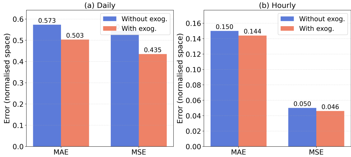
Figure 5.8: Forecasting performance comparison across temporal resolutions. Panel (a) shows Daily resolution with MAE and MSE for models with and without exogenous features. Panel (b) shows Hourly resolution with MAE and MSE. Hourly models achieve lower absolute error while daily models show larger relative improvements from exogenous features.
