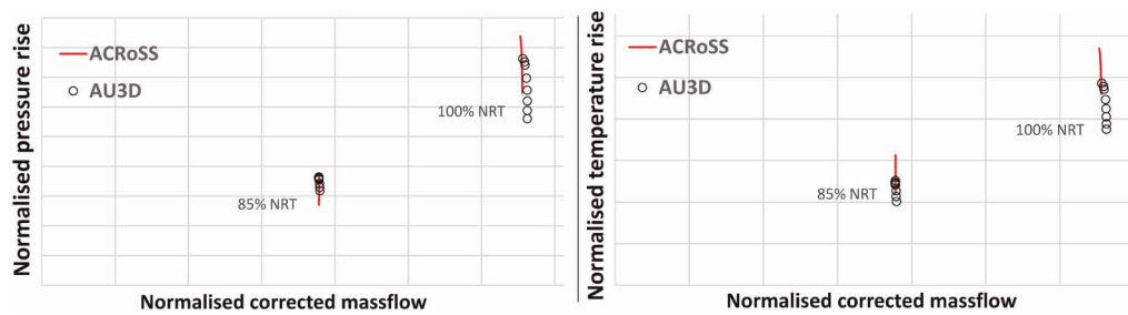
Figure 5. Comparison of un-stalled characteristics predicted by AU3D and ACroSS.
