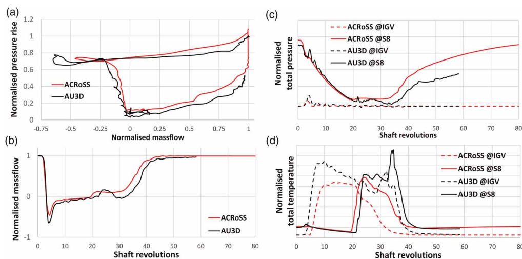
Figure 6. Comparison of transient event time histories during surge at 85% speed from ACroSS and AU3D. Compressor map (a), massflow at IGv inlet (b), total pressure (c) and total temperature (d) at IGv inlet and stator 8 outlet.
