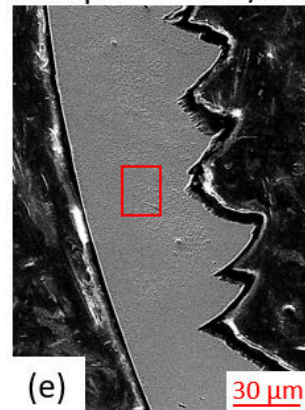
Fig. 13. – Chips cross-sections and EBSD orientation maps for (a,b) flood – 150 m/min, (c,d) 1000 psi – 150 m/min and (e,f) 1000 psi – 250 m/min.
