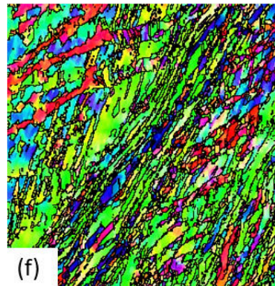
Fig. 13. – Chips cross-sections and EBSD orientation maps for (a,b) flood – 150 m/min, (c,d) 1000 psi – 150 m/min and (e,f) 1000 psi – 250 m/min.
