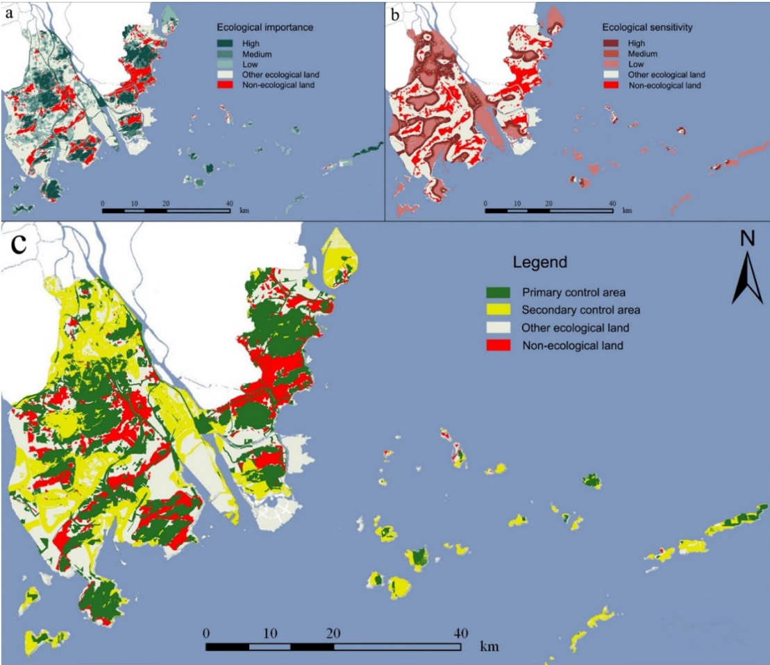
Figure 6 Management zoning for urban ecological land in Zhuhai City. a) Ecological importance; b) Ecological sensitivity; c) Management zoning
