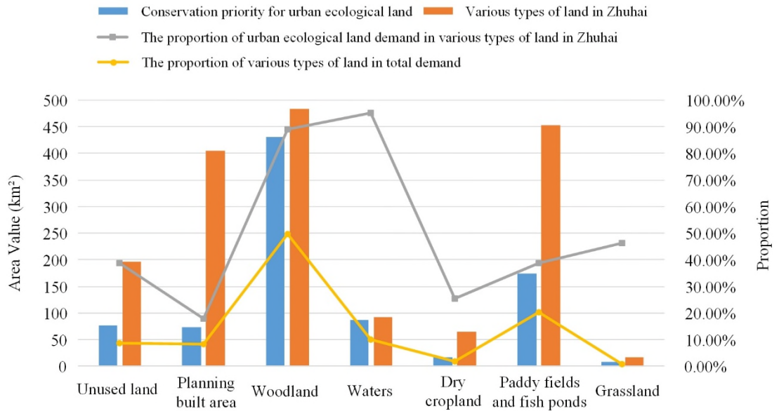
Figure 7 Area proportion contrast of land use types in the conservation priority area
