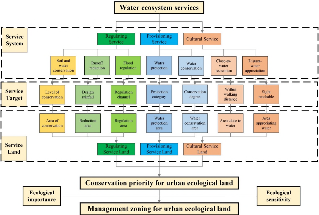
Figure 2 Research framework for identifying the conservation priority area and management zoning for urban ecological land
