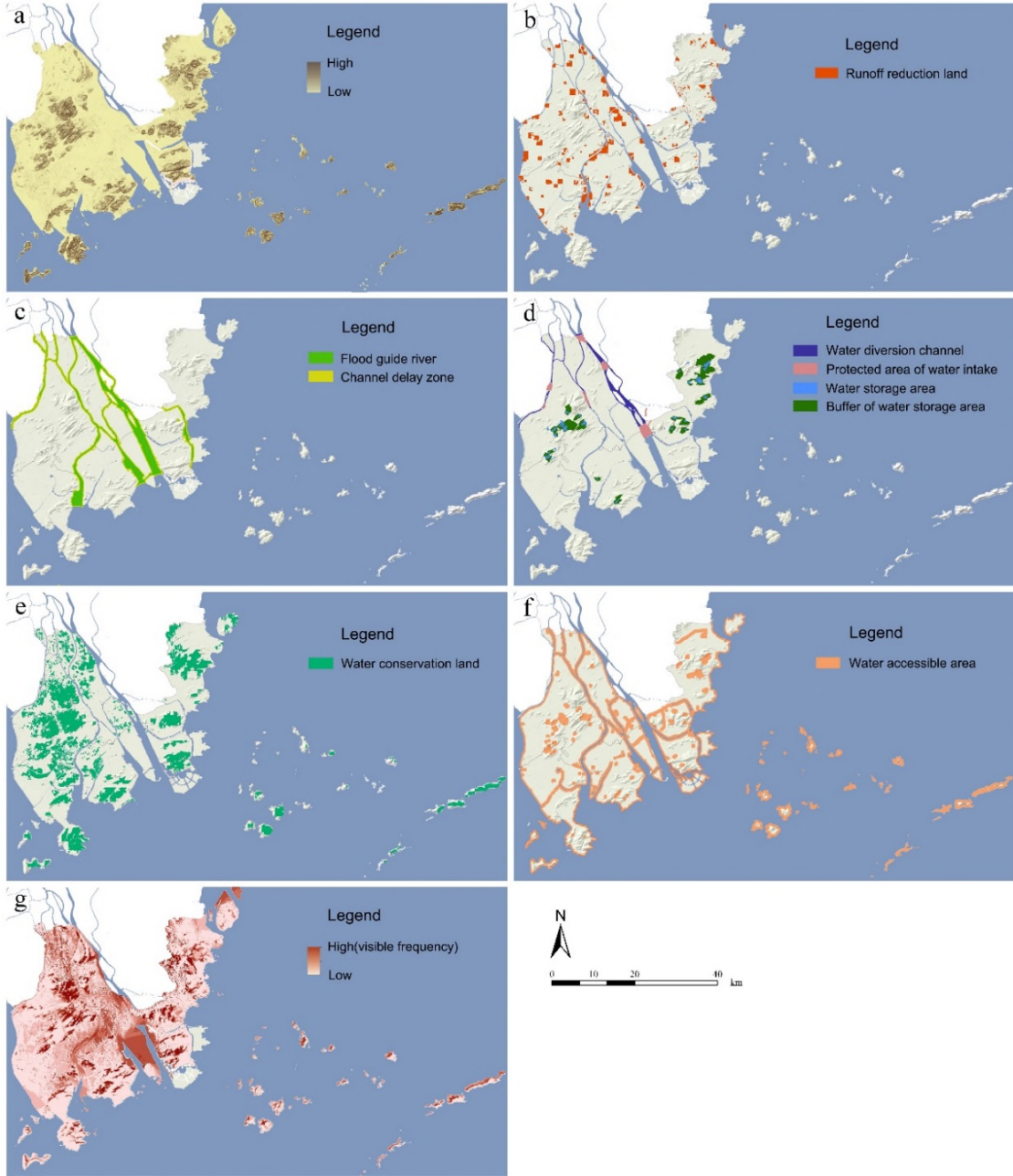
Figure 3 Spatial distribution of key areas for water ecosystem services in Zhuhai City. a) Soil retention area; b) Runoff reduction area; c) Flood regulation area; d) Water protection area; e) Water conservation area; f) Water recreation area; g) Water appreciation area.
