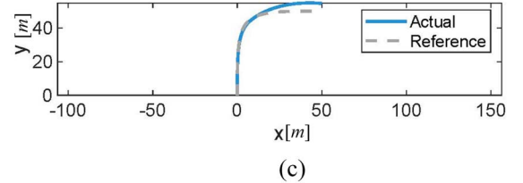
Fig. 11: Tracking performance in BT experiments at (a) 1m/s (b) 10m/s (c) 15m/s
