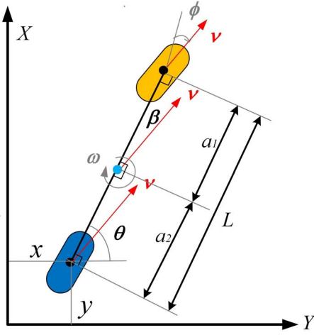
Fig. 1: Lateral dynamic of vehicle model
