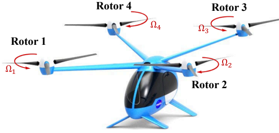
Figure 4 Single-passenger quadrotor aircraft [37].
