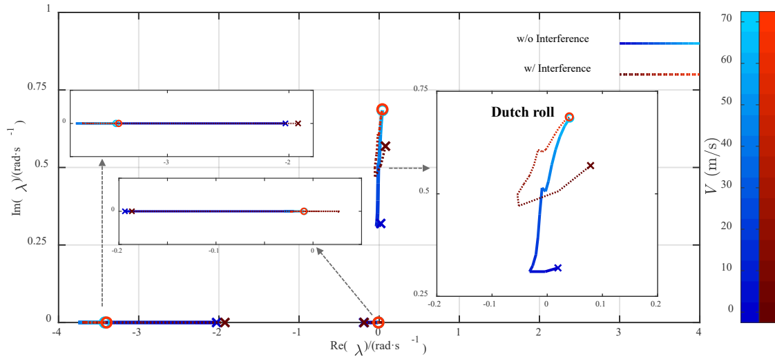
Figure 17 Root locus distribution of lateral-directional modes with flight speed.
