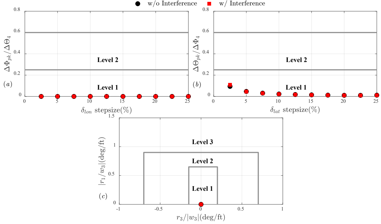
Figure 22 Cross-axis coupling for (a) roll-pitch, (b) pitch-roll, and (c) yaw-heave interactions.
