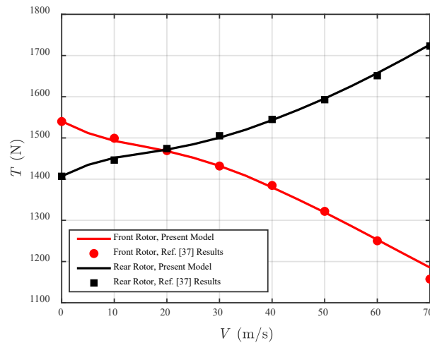
Figure 7 Comparison of front and rear rotor thrust variations with flight speed.
