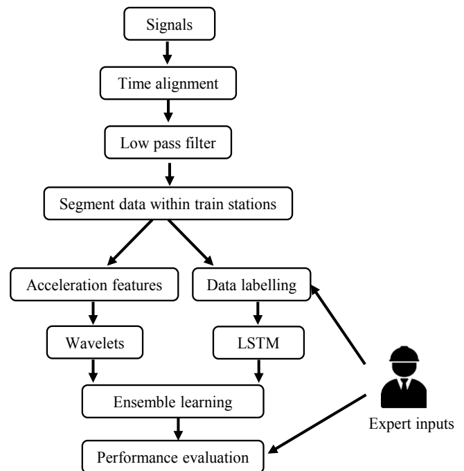
Figure 3 Methodology workflow
