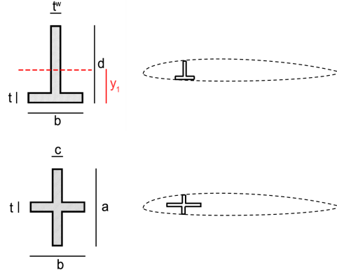
Fig. 4 Two different shapes were considered as spar cross section: (left) T-shape and (right) cross-shape.
