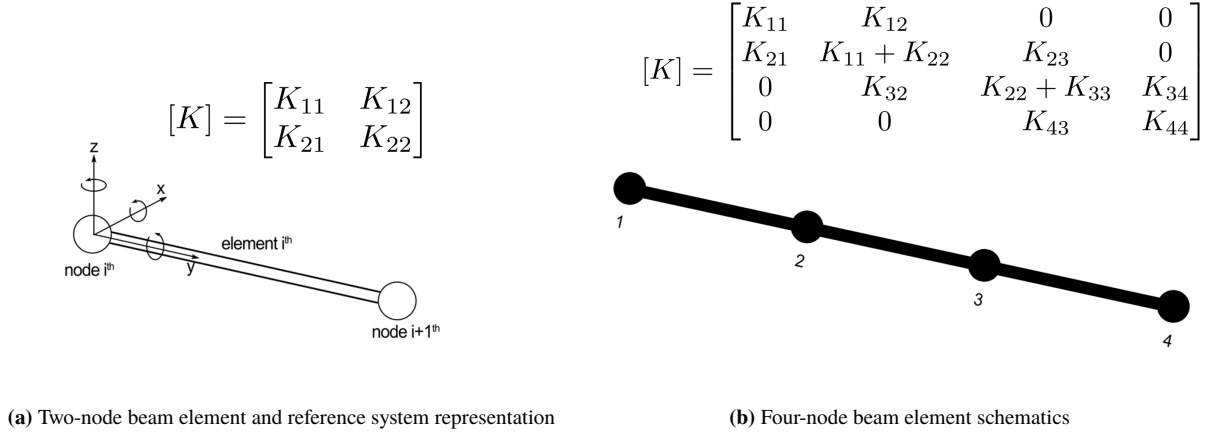
Fig. 3 Beam element
