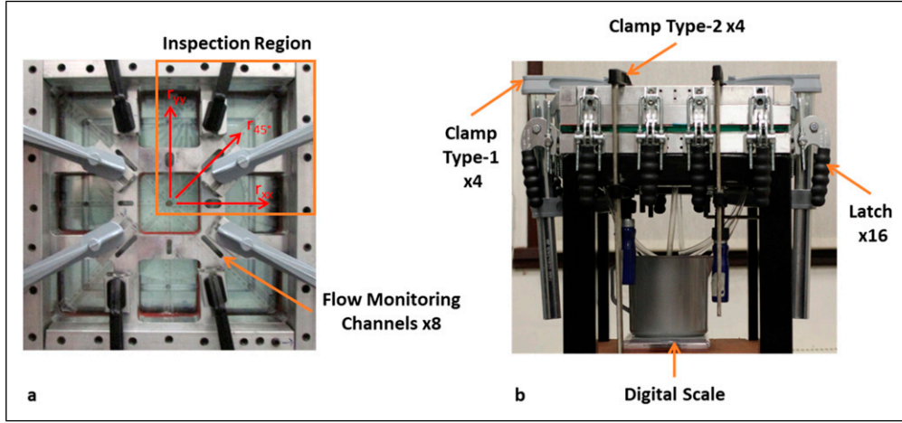
Figure 3. 2D (radial) permeability measurement setup: (a) top view and (b) side view.
