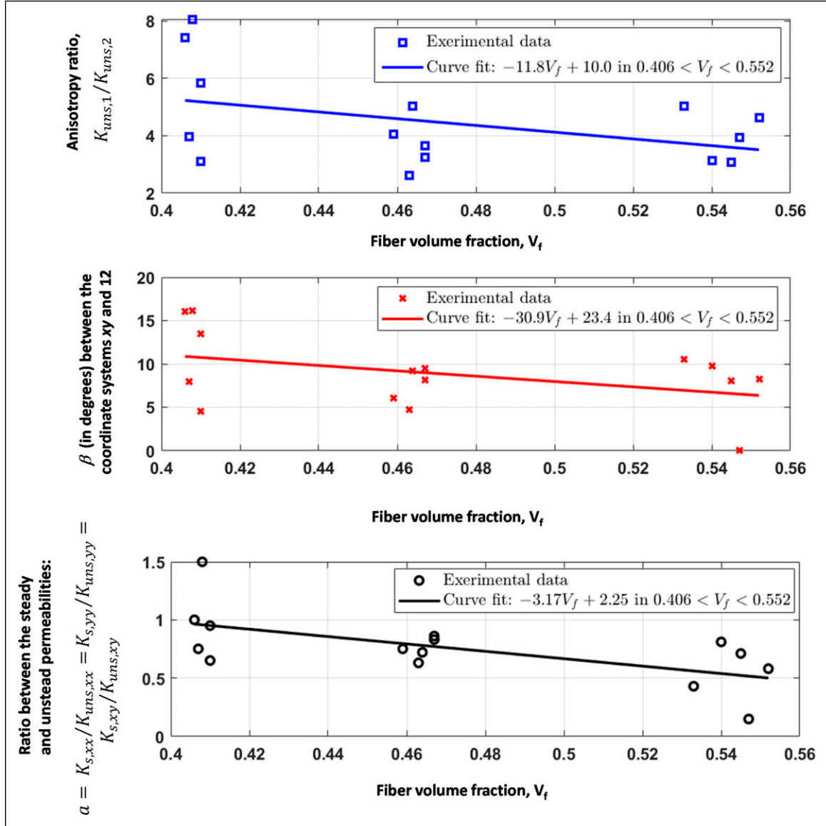
Figure 10. Analysis of the results; (top): anisotropy ratio, K_{uns,1}/K_{uns,2} ; (mid) the rotation angle, \beta between x - y and 1 - 2 coordinate planes; and (bottom) the ratio between the steady and unsteady permeabilities: a = \frac{K_{s,xx}}{K_{uns,xx}} = \frac{K_{s,yy}}{K_{uns,yy}} = \frac{K_{s,xy}}{K_{uns,xy}}
