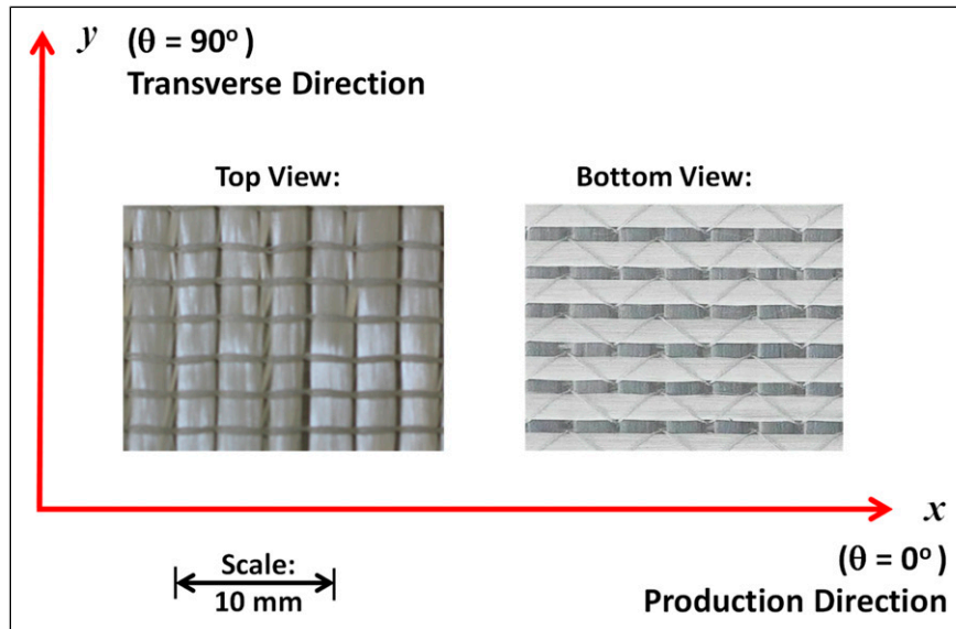
Figure 1. Top and bottom views of Metyx LT850 0/90 E-glass biaxial stitched fabric.
