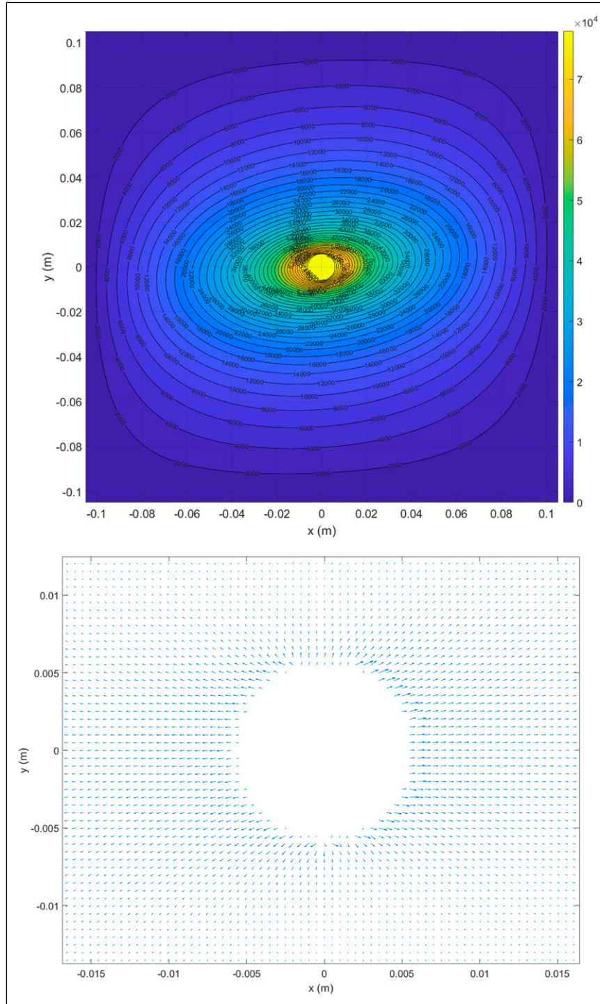
Figure 11. Numerically determined steady-state pressure distribution, P(x,y) in Pascals (top) and velocity field (bottom; around the inlet hole was shown here) for Experiment 7.
