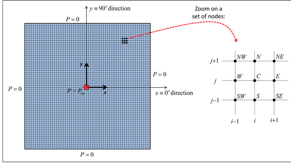
Figure 7. Grid and representative nodes used in finite difference method. Here a coarse mesh was illustrated, however, a finer grid with N_x = N_y = 421 (i.e., \Delta x = \Delta y = H = \frac{0.210\text{ m}}{421-1} = 0.0005\text{ m} ) was used in all simulations. The representative nodes were named as C (Central), W (West), E (East), N (North), South (S), NW (North West), and so on.
