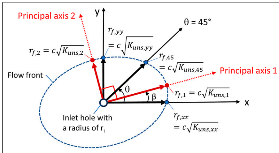
Figure 4. Coordinate systems x – y and 1–2. The three radii r_{f,xx} , r_{f,45^\circ} and r_{f,yy} of the elliptical flow front are tracked and used to calculate the unsteady permeability components K_{uns,xx} , K_{uns,45^\circ} and K_{uns,yy} , along x , \theta = 45^\circ and y directions, respectively.
