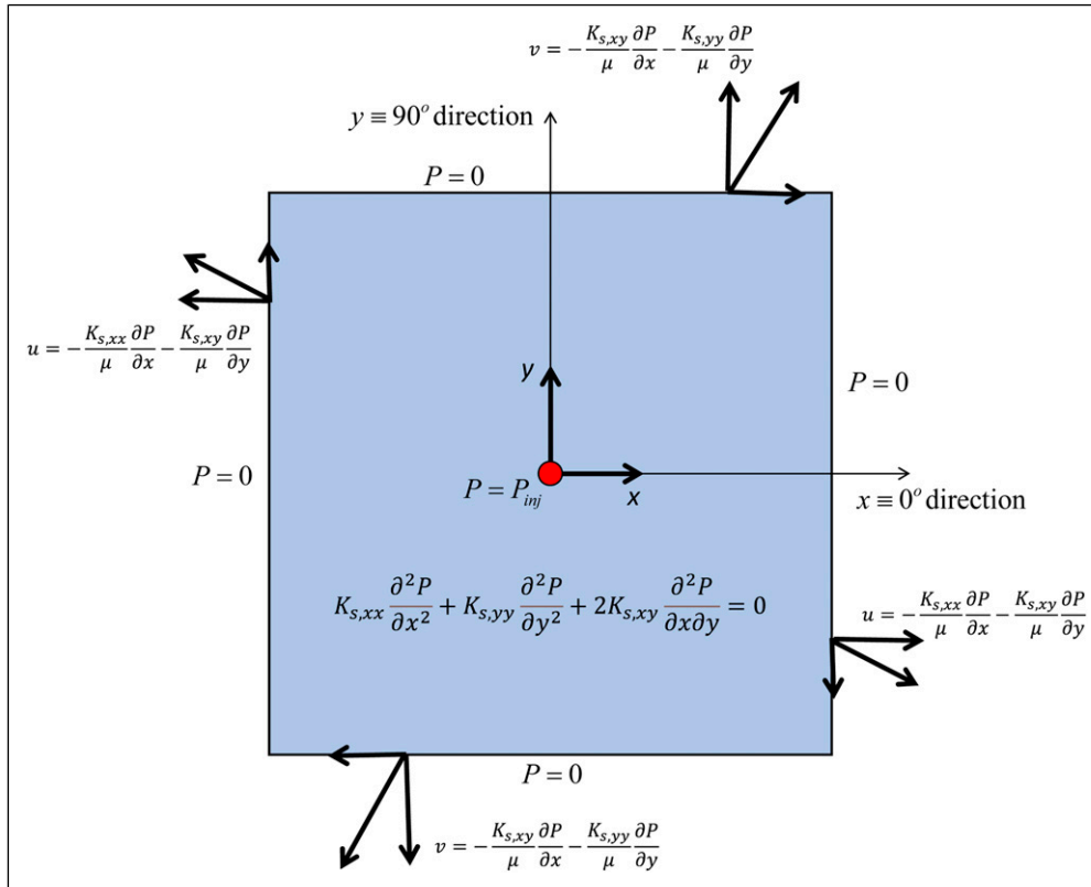
Figure 6. The domain of the fabric specimen wetted with resin at steady state 2D flow. Pressure boundary conditions were defined at the inlet hole and the outer periphery. Normal exit velocity components were specifically shown here and used to compute outflow rate at steady state.
