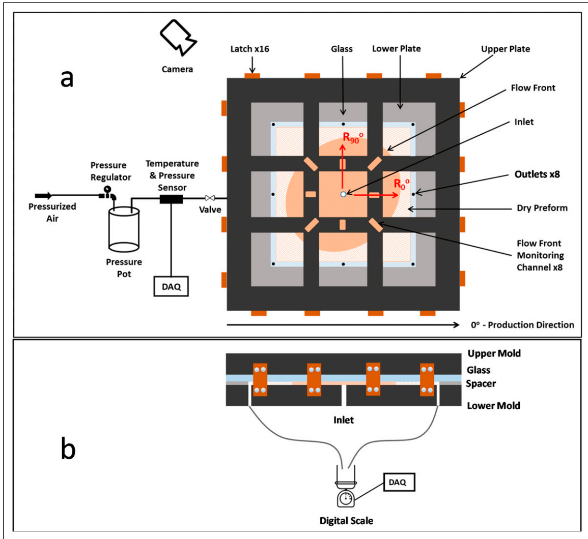
Figure 2. 2D (radial) permeability measurement setup: (a) top view and (b) side view. Transient (unsteady) flow regime is illustrated here where the elliptical flow front has not reached the exit pool along the mold edges yet.
