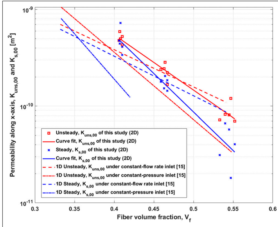
Figure 13. Comparison of the results from this study for 5-layer specimens under 2D (radial) experiments with those from a previous study by Yalcinkaya et al. 15 for 8-layer specimens under 1D experiments, using the same fabric. Note that only the permeability component along the x-axis was compared, as their analysis was conducted exclusively in that direction.
