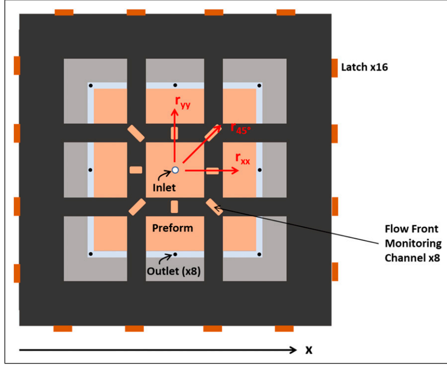
Figure 5. Top view of the 2D (radial) permeability measurement setup schematically showcasing a steady flow regime, i.e., when the fabric preform was fully wetted.
