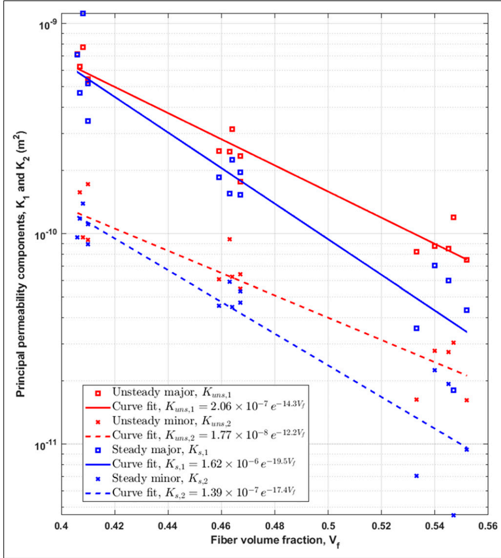
Figure 12. Principal components of unsteady and steady permeabilities of the fabric preform.
