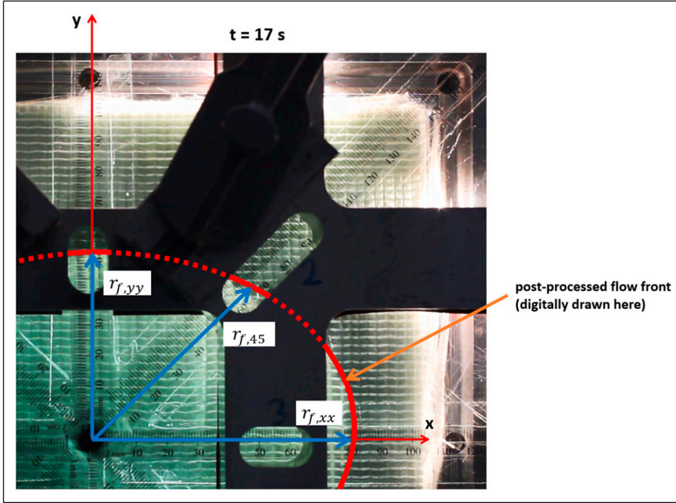
Figure 8. Elliptical flow front of resin at a sample instant.
