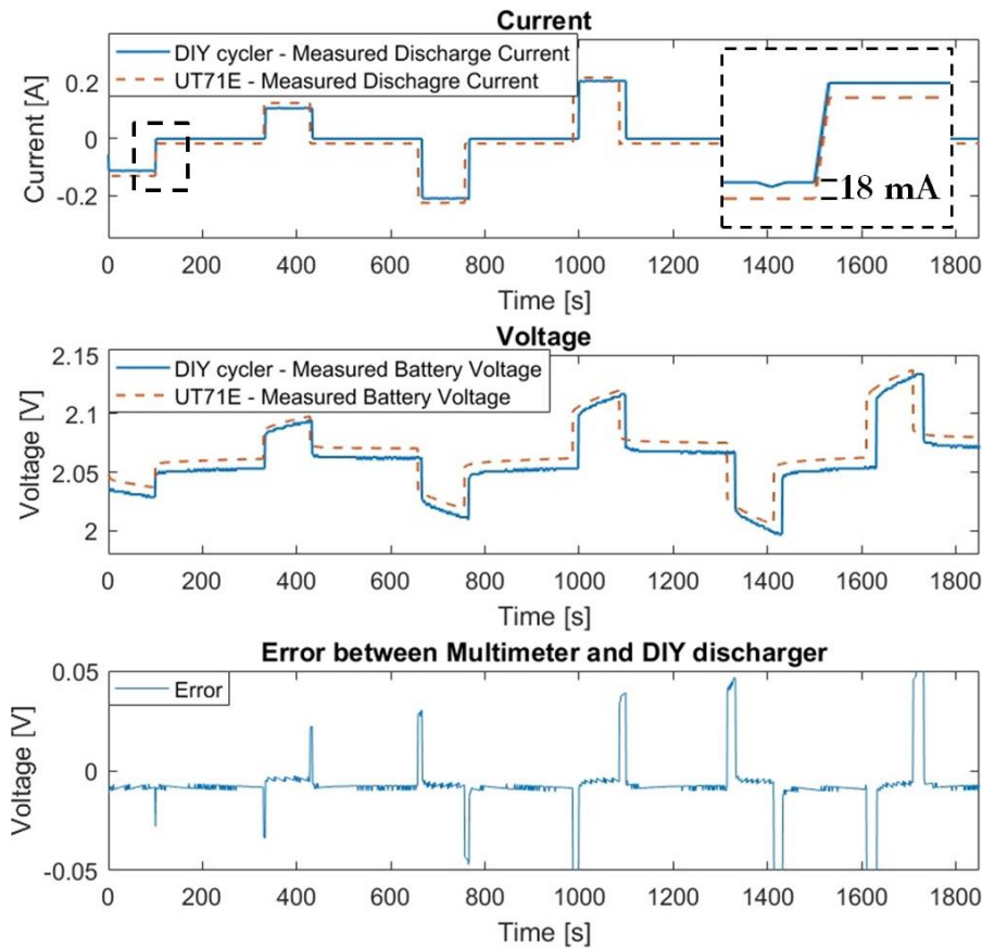
Figure 9 Voltage and current measurements of the Uni-T 71E and the Arduino cyclers
