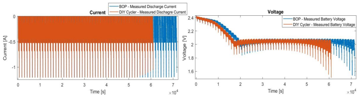
Figure 7 Voltage and current measurements for the whole of the drive cycle test
