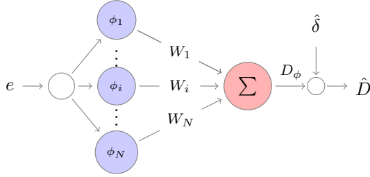
Fig. 2. RBF-NN structure.
