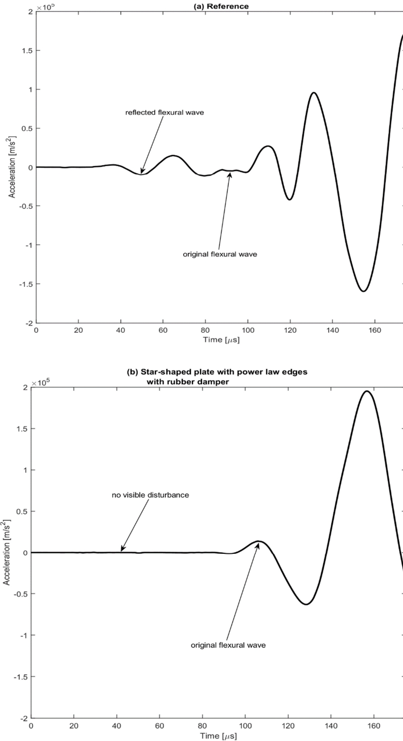
Figure 1-6: Acceleration signal acquired on (a) reference plate (b) star-shaped plate with power-law edges with rubber damper. This picture shows the benefit of the power-law edge design, the steady increase without disturbances of the wave amplitude after impact. Disturbances that can be recognised in the case of the reference plate lead to an inaccurate AT detection.
