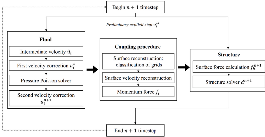
Fig. 6. Illustration of the FSI workflow.
