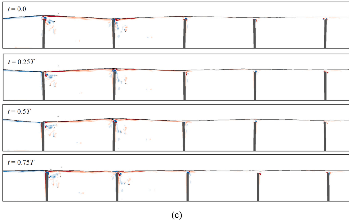
Fig. 17. Vorticity observation of cases with separation distance of \frac{d}{L} = 0.5 for various WEC number (a) N = 2 , (b) N = 3 , (c) N = 5 , (d) N = 7 .
