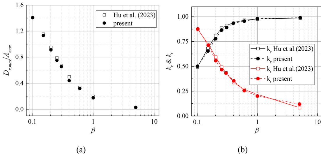
Fig. 9. Comparison of the present model with experimental results [33]. (a) Beam deflection at the free end, (b) Wave reflection and transmission for different structural stiffnesses \beta .
