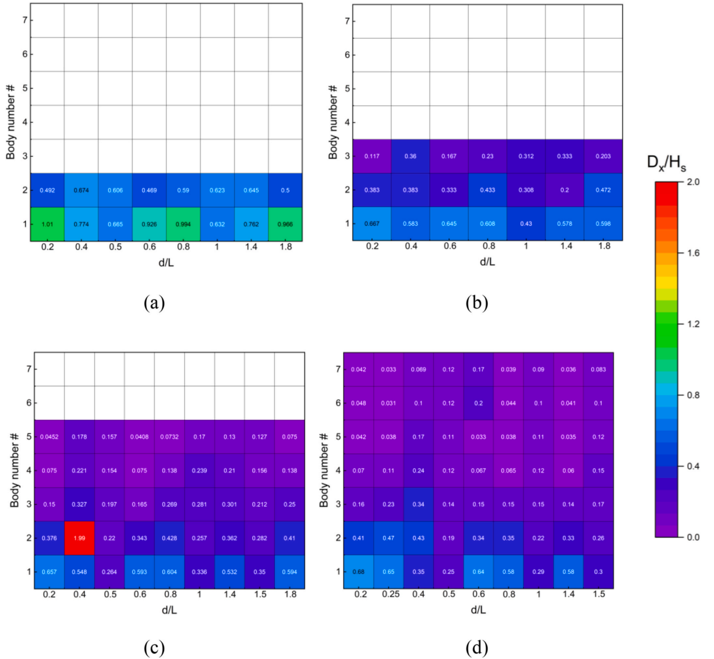
Fig. 19. Non-dimensionalised horizontal structural deformation D_x/H_s of each body with various separating distances and device numbers (a) N = 2 , (b) N = 3 , (c) N = 5 and (d) N = 7 .
