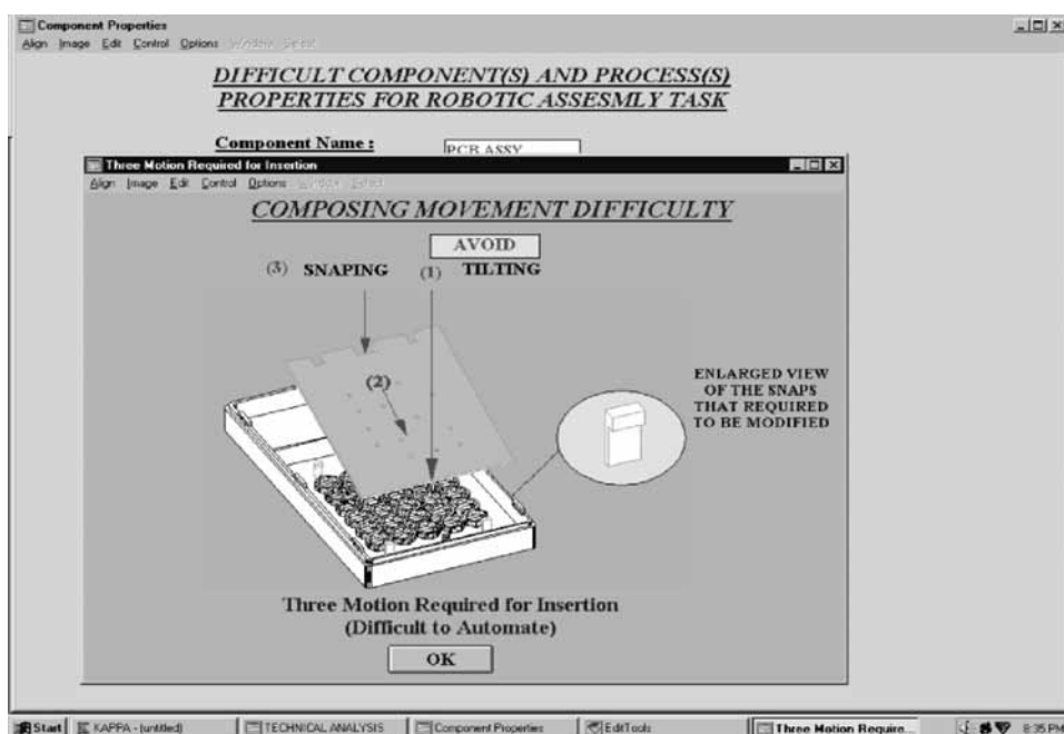
Fig. 14 The three motions required for insertion (difficult to automate)
