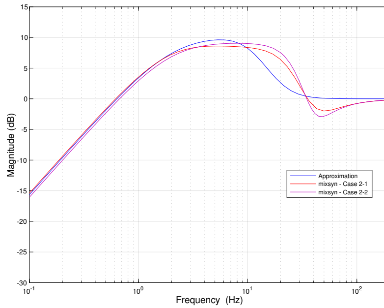
Fig. 8 Log-Magnitude of Sensitivity Frequency Response 20 \log_{10} |S(j\omega)| (Case 2)
