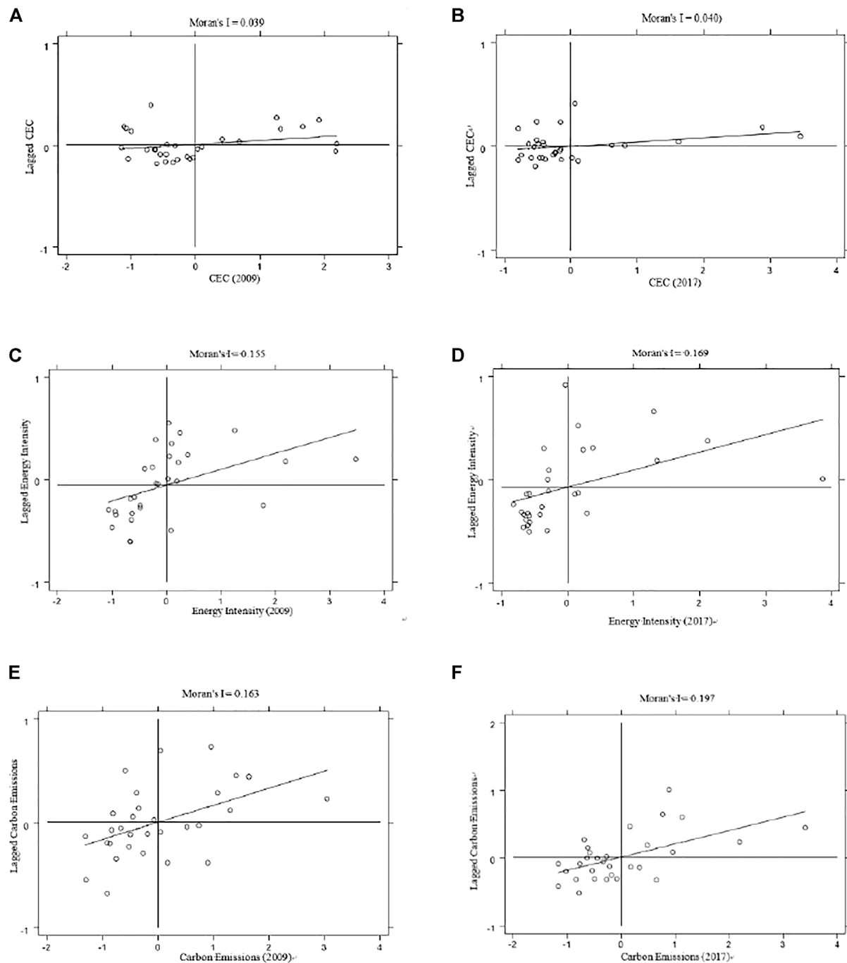
FIGURE 2 | Scatterplots of Moran's I of CEC, Energy intensity and Carbon emissions for 2009 and 2017.
