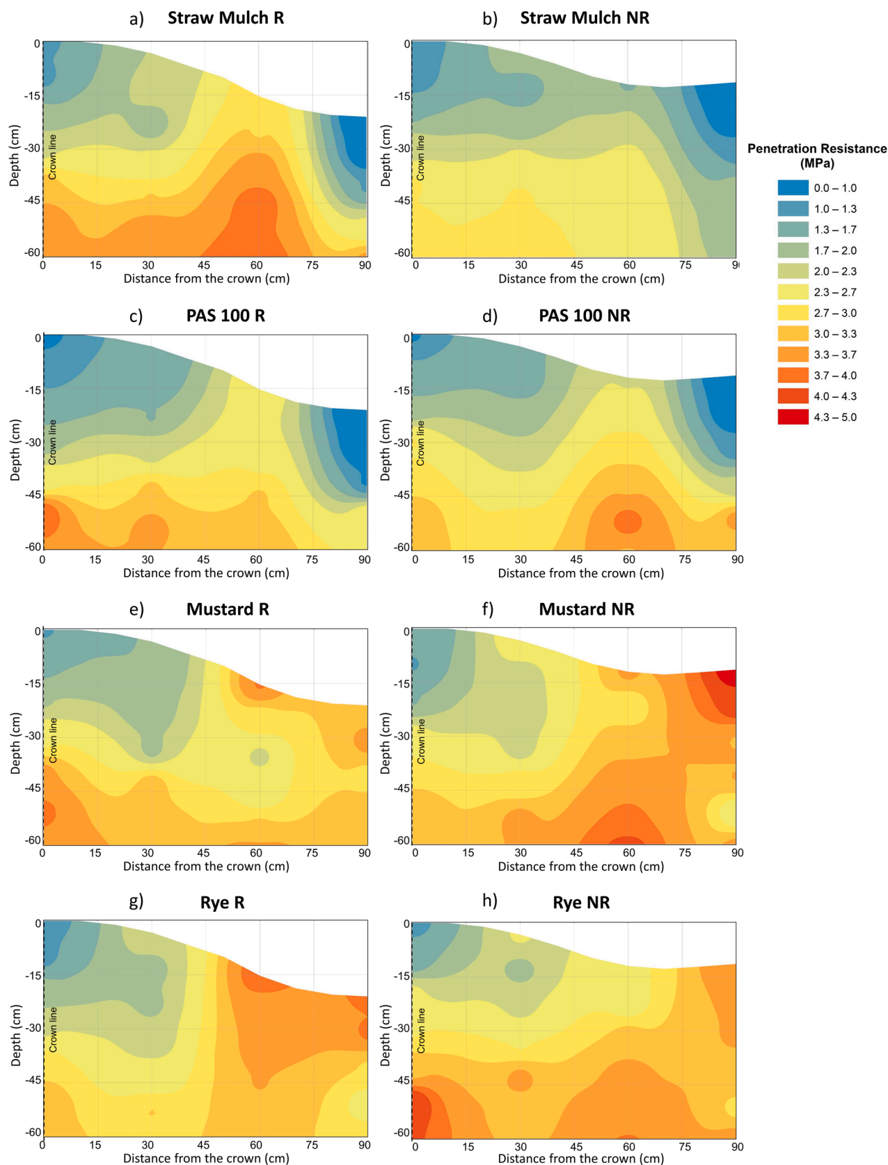
Fig. 7. 2020 mulch and companion crop treatments contour diagrams based on Penetration Resistance (MPa) determined at set positions from the crown line ( n = 4 ) using the inverse distance weighing (IDW) interpolation method.
