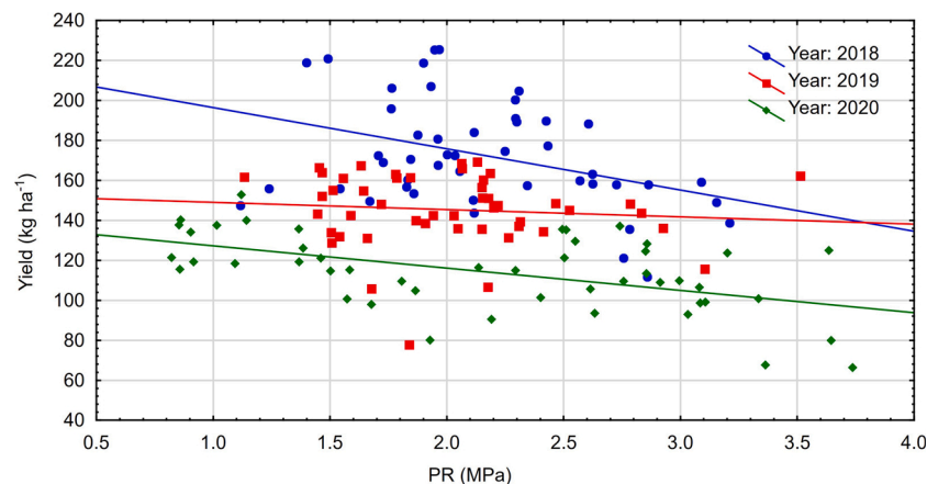
Fig. 8. Linear correlation between mean Penetration Resistance (MPa) in the centre of the asparagus interrow and asparagus yields ( \text{kg ha}^{-1} ). Points represent paired values obtained across all treatments. 2018: r^2 = 0.15 , r = -0.384 , p \leq 0.05 ; 2019: r^2 = 0.01 , r = -0.097 , p = \text{NS} ; 2020: r^2 = 0.15 , r = -0.381 , p \leq 0.05 . NS = Non-significant at 95% confidence interval.
