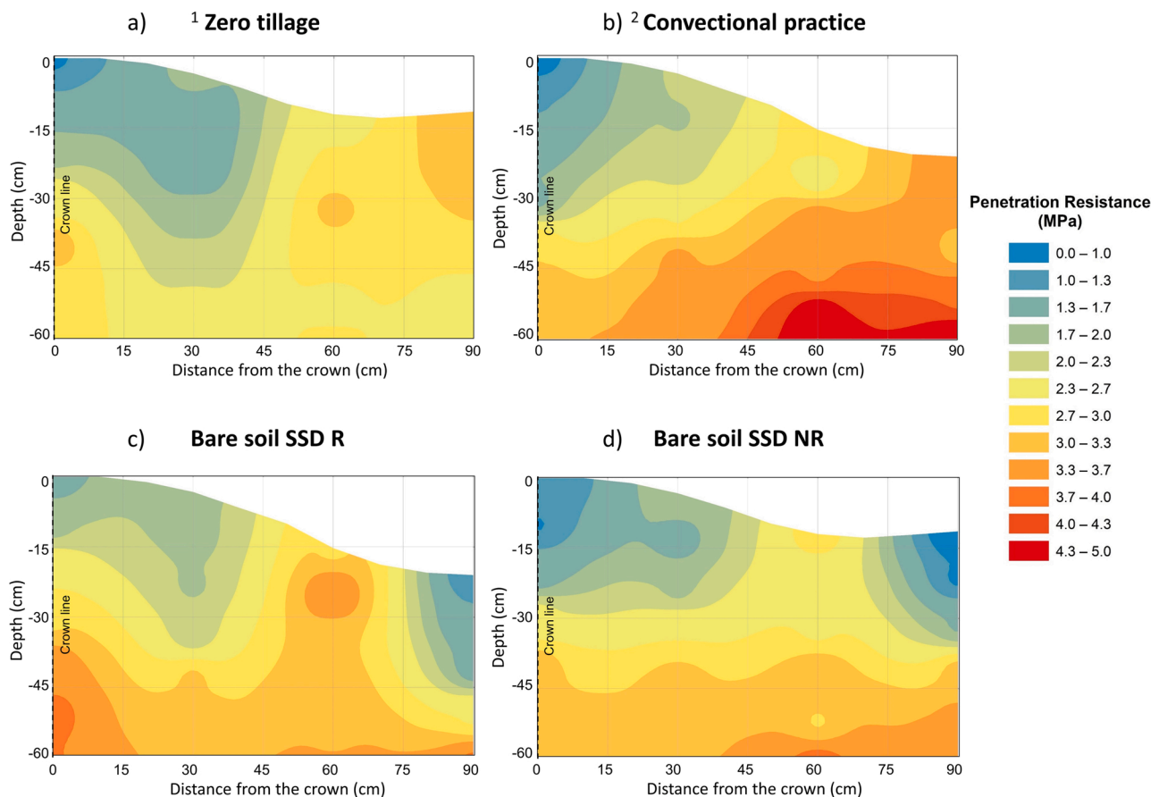
Fig. 6. 2020 bare soil treatments contour diagrams based on Penetration Resistance (MPa) transects determined tangential to the crown line ( n = 4 ) using the inverse distance weighing (IDW) interpolation method. 1 Bare soil No-SSD NR; 2 Bare soil No-SSD R.
