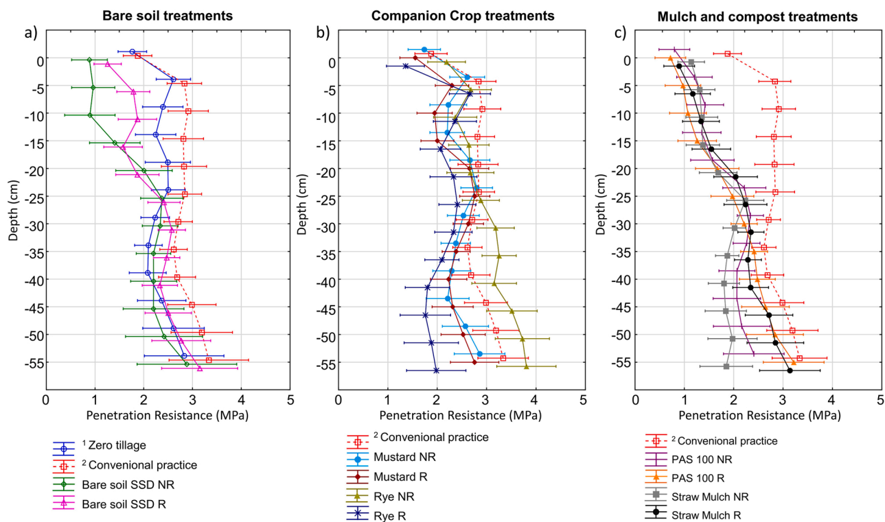
Fig. 3. Mean ( n = 12 ) 2018 Penetration Resistance (MPa) in the centre of the asparagus interrow at 5 cm depth intervals. Horizontal bars denote 0.95 confidence interval. 1 Bare soil No-SSD NR; 2 Bare soil No-SSD R.
