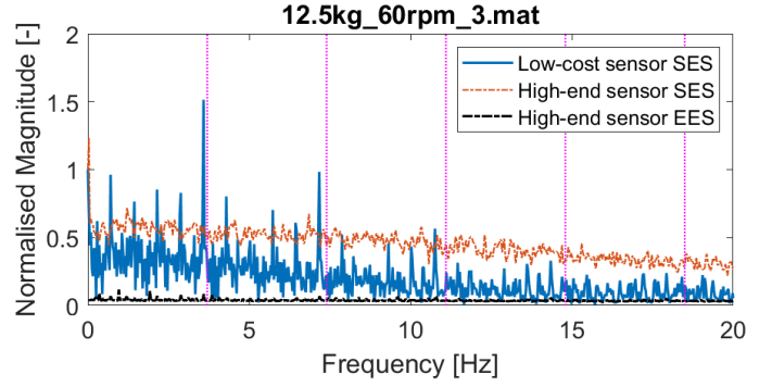
Figure 17: Envelope spectra of the outer race damaged bearing under 12.5 kg radial load and 60 rpm shaft speed obtained from the low-cost and high-end sensor signals.
