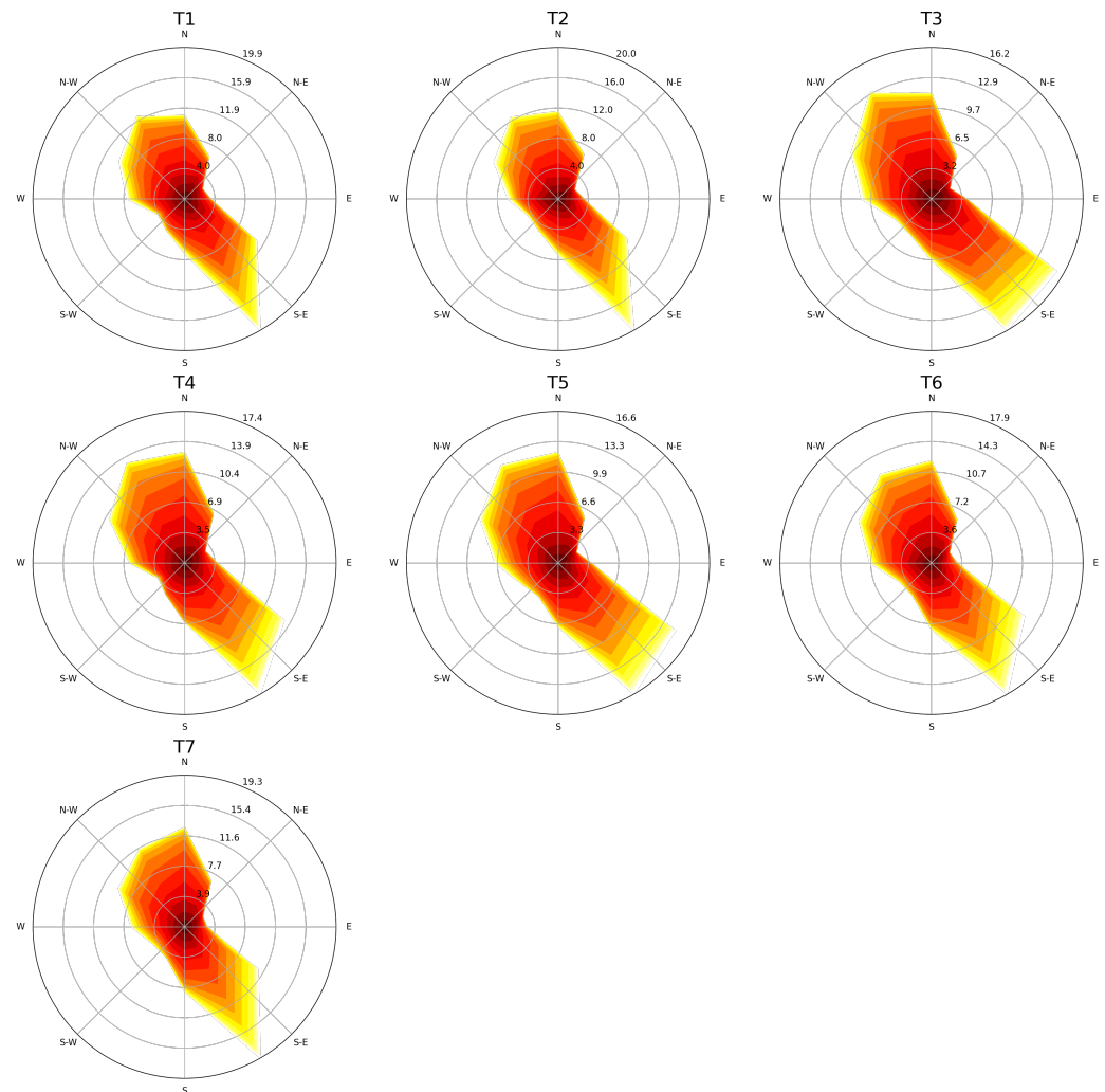
Figure 5. Wind speed directional distributions on the turbines.
