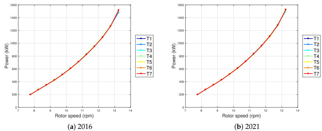
Figure 10. Rotor speed–power curve for the whole wind farm, computed using the binning method.
