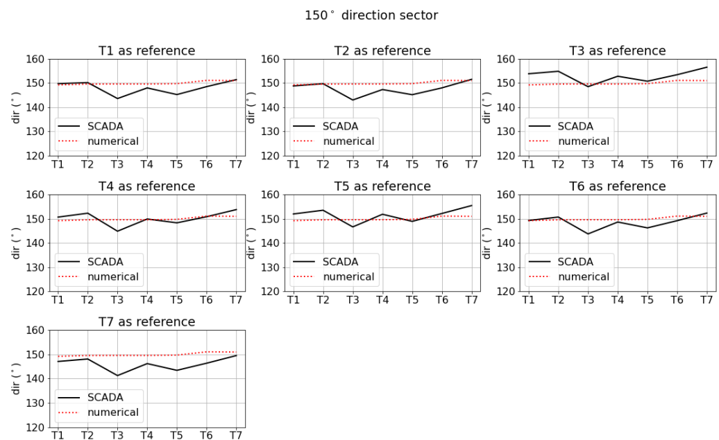
Figure 19. Comparison between simulation and measurements regarding the average wind direction, where each wind turbine is selected iteratively for tuning the model.
