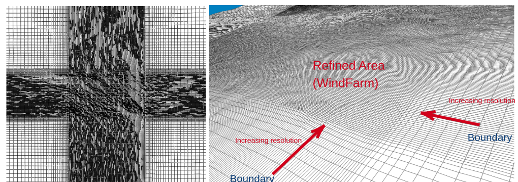
Figure 4. Grid resolution in the horizontal plane: from the boundary to the investigated area (WindFarm), the spacing is refined from 270 to 17 m.
