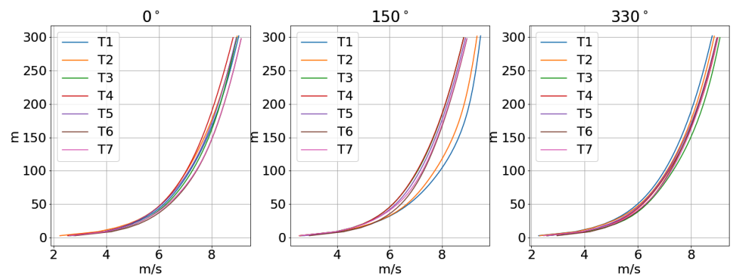
Figure 6. Wind speed profile for the 0°, 150°, and 330° direction sectors.
