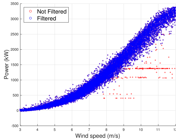
Figure 2. Example of raw and filtered power curve data of T1.
