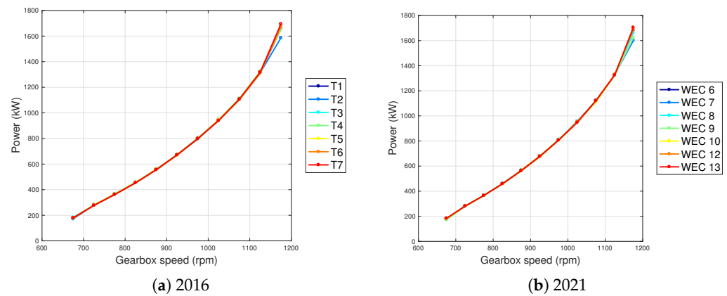
Figure 11. Gearbox speed–power curve for the whole wind farm, computed using the binning method.
