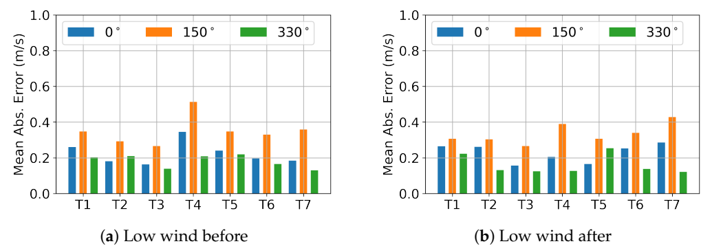
Figure 17. The mean absolute error between simulation and measurements for the sectors 0^\circ , 150^\circ and 330^\circ , before and after the replacement of the T4 nacelle anemometer: low wind regime.
