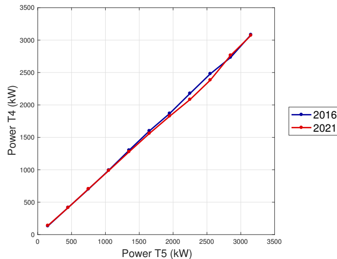
Figure 13. Power of T4 as a function of the power of T5, computed using the binning method: 2016 and 2021.
