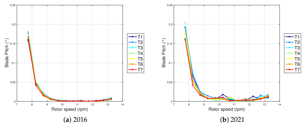
Figure 12. Rotor speed–blade pitch curve for the whole wind farm, computed using the binning method.
