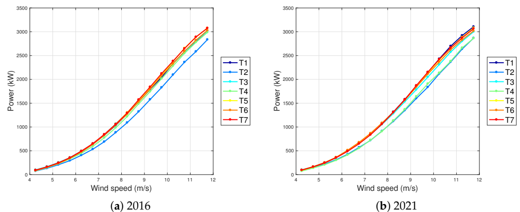
Figure 8. Power curve for the whole wind farm, computed using the binning method.
