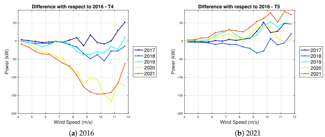
Figure 9. Difference of the power curve with respect to 2016, for wind turbines T4 and T5.
