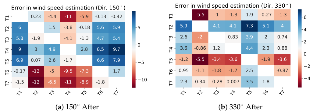
Figure 16. Percentage error in the wind speed estimation upon the replacement of the T4 nacelle anemometer: low wind regime. In the i -th row, the results are obtained by calibrating the model on the nacelle wind speed of the i -th wind turbine.
