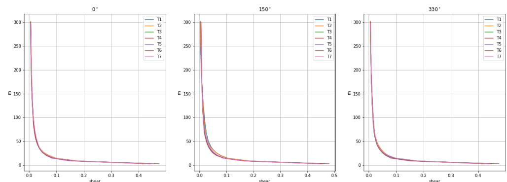
Figure 7. Wind shear profile for the 0°, 150°, and 330° direction sectors.
