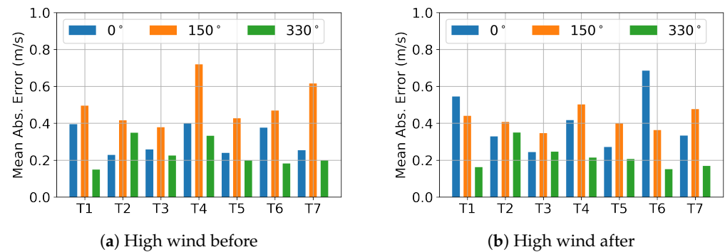
Figure 18. The mean absolute error between simulation and measurements for the sectors 0^\circ , 150^\circ and 330^\circ , before and after the replacement of the T4 nacelle anemometer: high wind regime.
