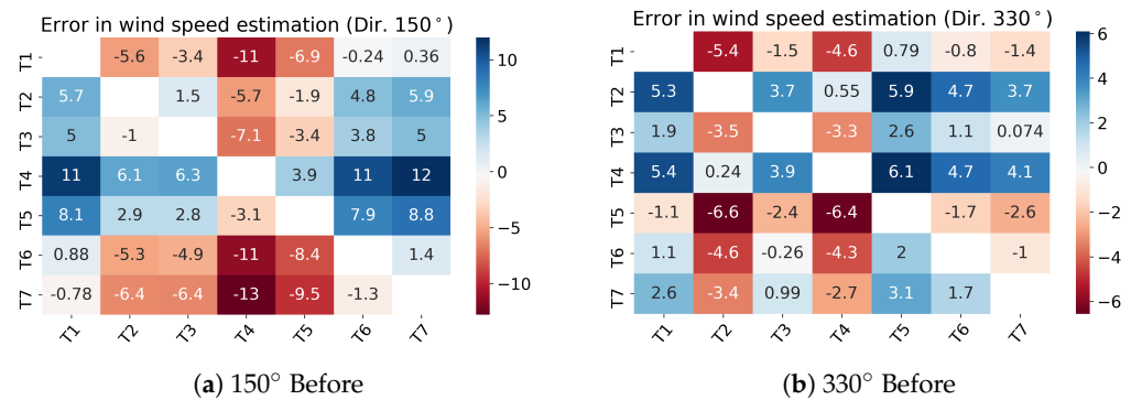
Figure 15. Percentage error in the wind speed estimation before the replacement of the T4 nacelle anemometer: low wind regime. In the i -th row, the results are obtained by calibrating the model on the nacelle wind speed of the i -th wind turbine.
