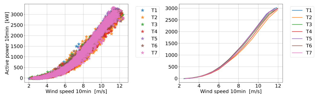
Figure 14. Power curve for the whole wind farm, computed using the binning method: 2022, upon nacelle anemometer replacement at wind turbine T4.
