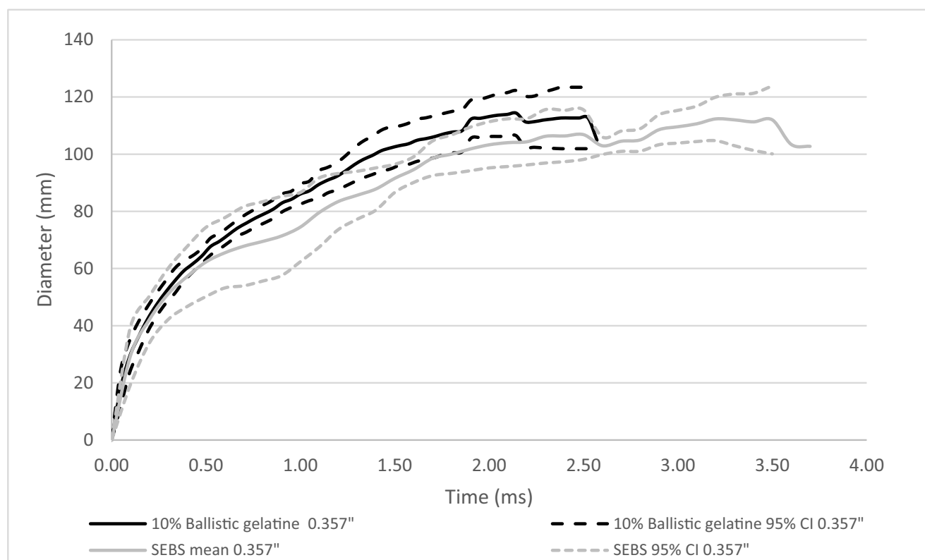
Fig. 7 Comparison of dynamic BFS mean diameter with 95% confidence intervals (95% CI) on SEBS gel and 10% ballistic gelatine – 0.357'' projectile
