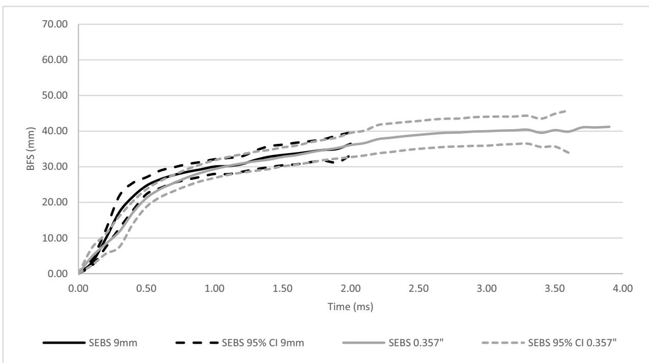
Fig. 5 Comparison of 9 mm and 0.357\"/>
