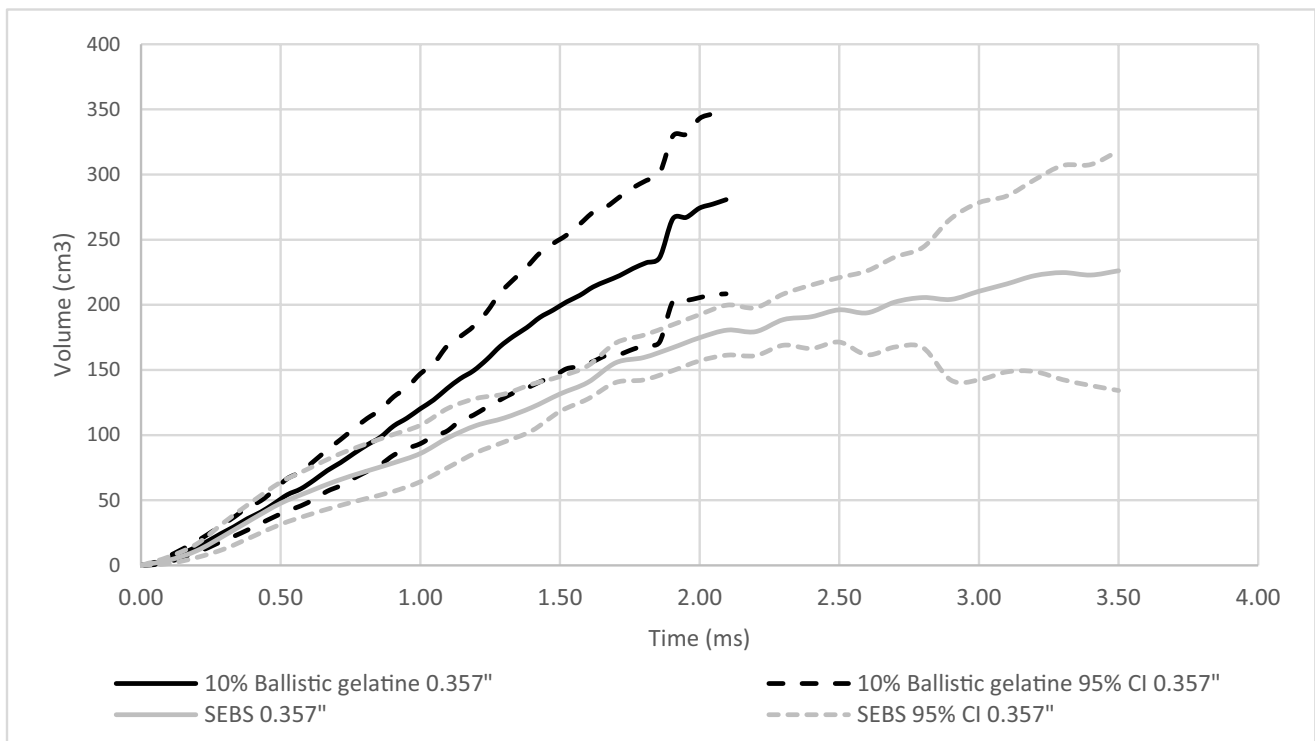
Fig. 9 Comparison between SEBS gel and 10% ballistic gelatine of dynamic BFS mean estimated volume of BFS with 95% confidence intervals (95% CI) for 0.357"
