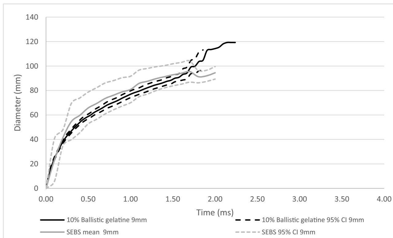
Fig. 6 Comparison of dynamic BFS mean diameter with 95% confidence intervals (95% CI) on SEBS gel and 10% ballistic gelatine– 9 mm projectile
