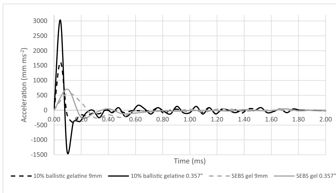
Fig. 10 Acceleration of BFS mean depth in 10% ballistic gelatine and SEBS gel in response to impacts on armour panels from 9 mm and 0.357” projectiles
