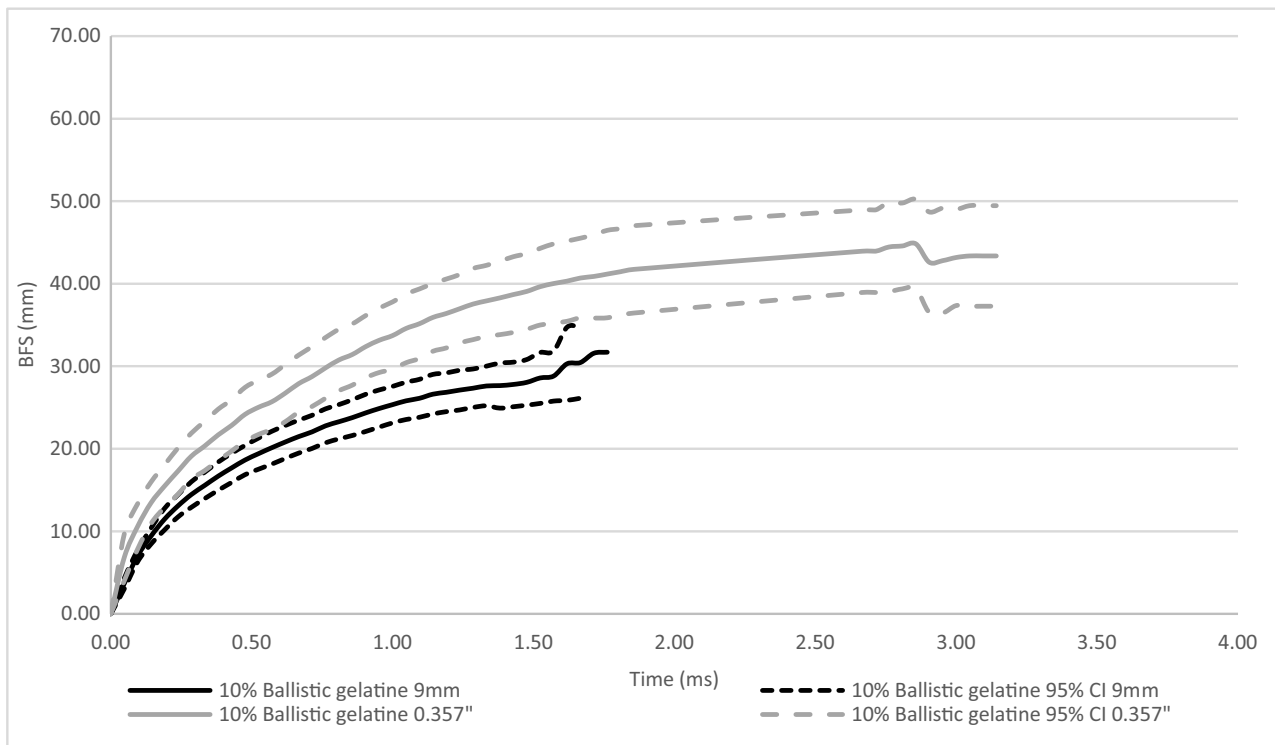
Fig. 4 Comparison of 9 mm and 0.357\"/>
