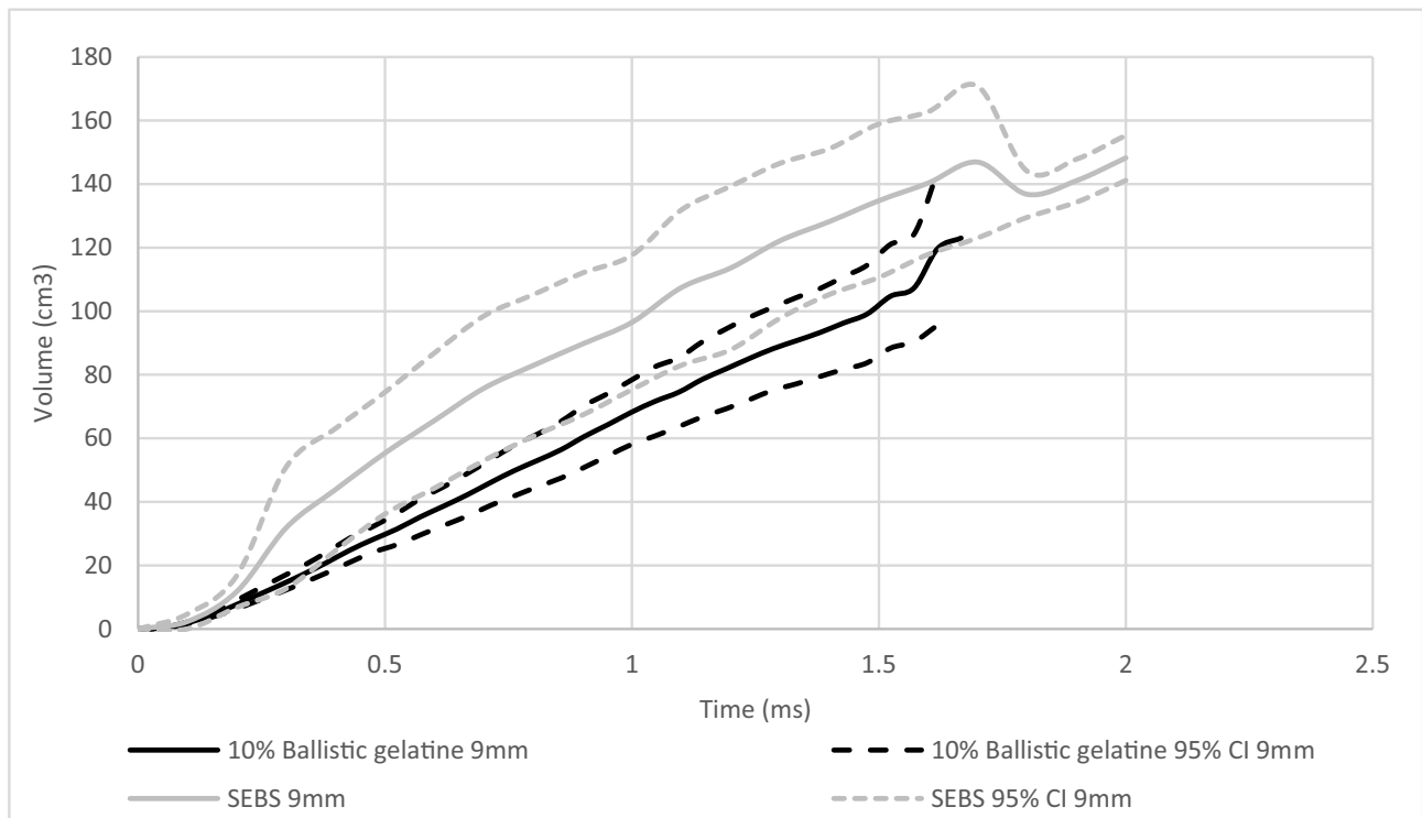
Fig. 8 Comparison between SEBS gel and 10% ballistic gelatine of dynamic BFS mean estimated volume of BFS with 95% confidence intervals (95% CI) for 9 mm
