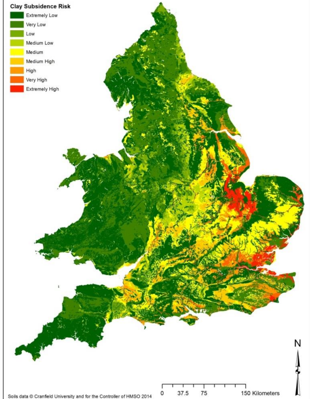
Figure 2: Natural Perils Directory Clay subsidence risk model, based upon annual mean potential soil moisture deficit (1961-75 baseline).
