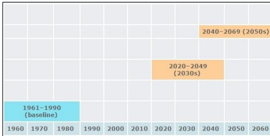
Figure 4: The UKCP09 climatic probabilistic scenarios considered within this research (modified from: http://ukclimateprojections.metoffice.gov.uk )
