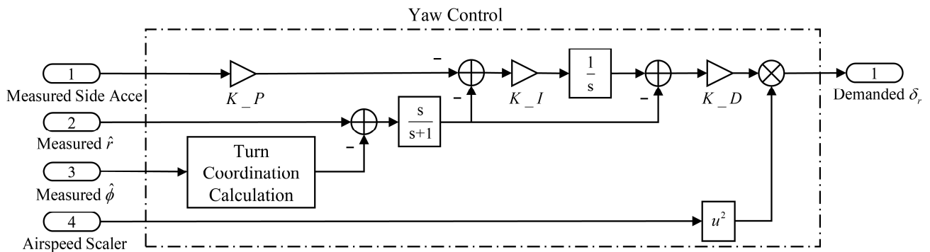
Figure 8. Yaw control loop schematic diagram.
