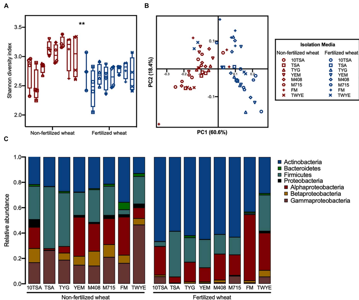
FIGURE 3 | Influence of different culture-agar on bacterial community diversity and structure in the rhizosphere of wheat grown in soils with and without fertilizer. (A) Alpha diversity estimates at ASV level for rhizosphere bacterial communities grown on eight agar types with median (line) and hinges at first and third quartiles (25th and 75th percentiles). Significant differences as determined by two-way type III ANOVA are shown by “****” for p < 0.01 between treatment groups. (B) PCoA plot of bacterial community composition based on weighted UniFrac distances at ASV level, colored by fertilizer treatment. Symbols represent the isolation media that bacteria were cultured on from rhizosphere samples: TSA (10th concentration) (circles), TSA (squares), TYG (up-triangles), YEM (down-triangles), M408 (diamond), M715 (hexagon), FM (plus), TWYE (cross). (C) Average relative abundances of bacterial phyla within the bacterial 16S V3–V4 sequences. Identifications are based on the SILVA database for prokaryotes.
