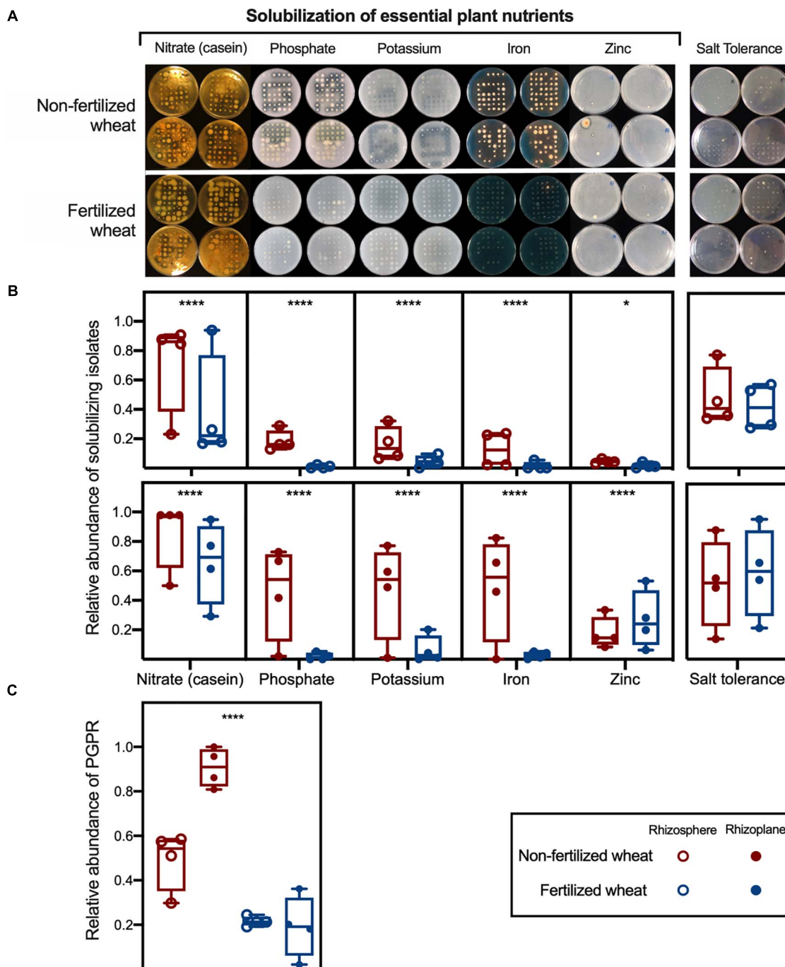
FIGURE 4 | Relative abundance of culturable rhizobacteria with plant growth-promoting traits isolated from wheat grown in soils with and without fertilizer. (A) Nitrate-, phosphate-, potassium-, iron-, and zinc-solubilization as determined by casein, PVK, AVK, CAS, and zinc carbonate agar, respectively. Casein, phosphate, potassium, and zinc solubilization are indicated by clear halos surrounding the colony whereas orange halos indicate iron solubilization. Salt tolerance as determined by 10TSA supplemented with 5% NaCl. Box plots show relative abundance of (B) solubilizing isolates and salt tolerant isolates and (C) relative abundance of PGPR isolates, as determined by functional bioassays; with median (line) and hinges at first and third quartiles (25th and 75th percentiles). Each point represents an isolate library ( n = 94 ) derived from rhizosphere (open circles) and rhizoplane (closed circles) samples. Single colonies were isolated from different non-selective agar and 10TSA respectively and inoculated in TSB (1/10th concentration) in a 96-well plate; sterile TSB (1/10th concentration) in 2× wells were left uninoculated to act as a negative control. Significant differences as determined by Chi-squared tests are shown by “*” and “****” for p < 0.05 and p < 0.0001 , respectively.
