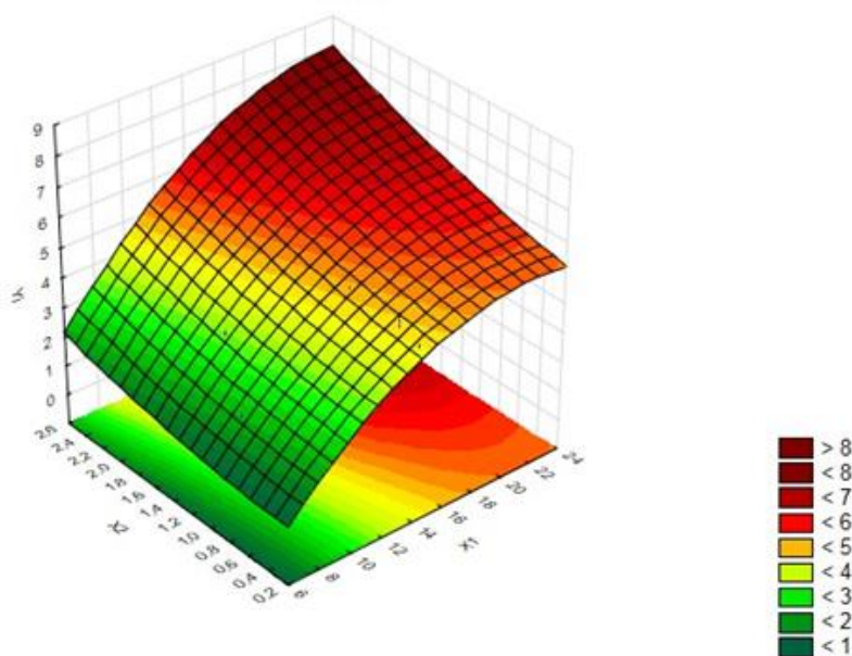
Figure 2. Response surface of ethanol production as a function of the concentration of CWP and inoculum ratio of K. marxianus NCAIM Y0963 in mixed culture.
