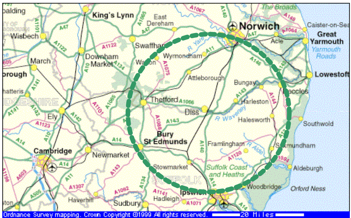
Figure 29. Map of Suffolk and Norfolk showing the potential catchment area included within a 40 km radius (●●●●) around the proposed renewable energy power station at Eye.
