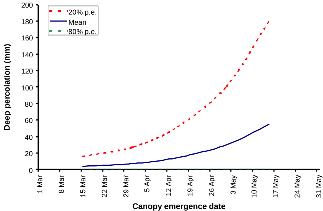
Figure 16. Effect of different canopy emergence dates on simulated deep percolation under willow SRC at Silsoe, Beds, showing the 20% and 80% probabilities of exceedence values.
