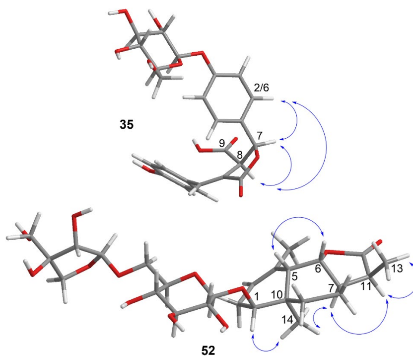
Fig. 4. Key NOESY correlations of compounds 35 and 52.
