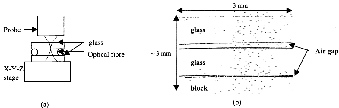
Figure 5: (a) Experimental set-up, showing position of the Rayleigh range relative to the sample and (b) 2D image formed from scans.
