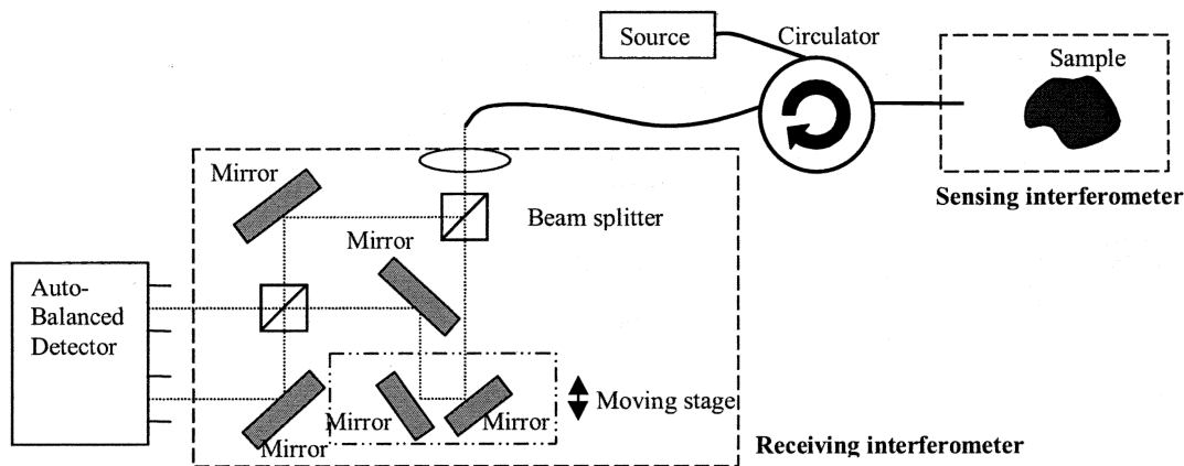
Figure 4: Fizeau configuration with a Mach-Zehnder receiving interferometer
