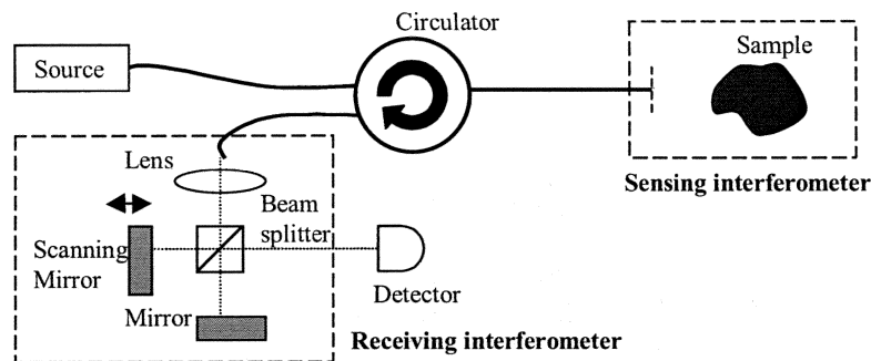
Figure 3: Fizeau configuration with a Michelson receiving interferometer
