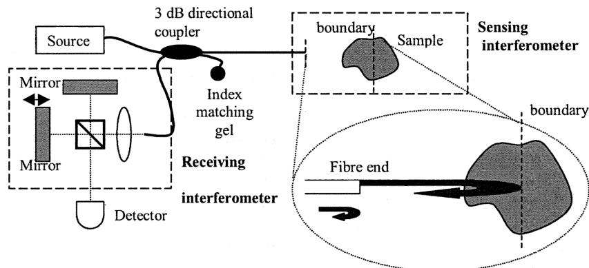
Figure 2: Fizeau interferometer configuration for OCT, based around a 3 dB directional coupler
