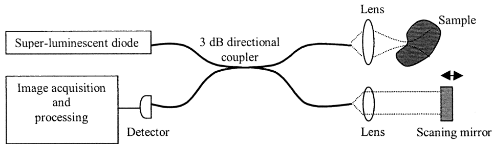
Figure 1: Fibre-coupled Michelson interferometer configuration for OCT.
