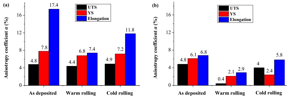
Fig.17 Anisotropy variation during tensile test after (a) standard SA and (b) HSA heat treatment
