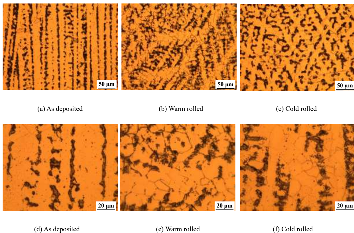
Fig.10 Microstructure of IN-718 after homogenization plus solution and double-aging heat treatment:
