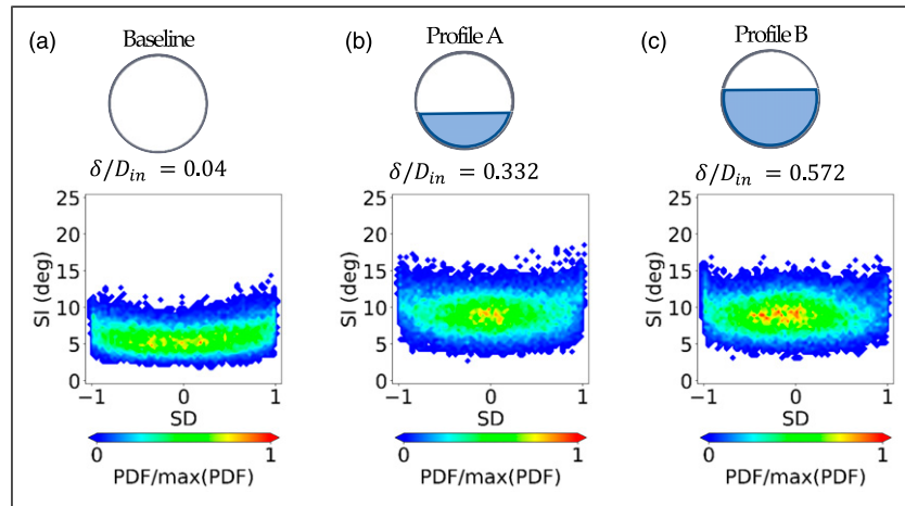
Figure 9. j-PDF of the SI-SD distributions measured at the AIP at r/R = 0.84 for different inlet conditions: baseline, Profile A and Profile B ( \delta/D_{in} = 0.04 , \delta/D_{in} = 0.332 and \delta/D_{in} = 0.572 , respectively).
