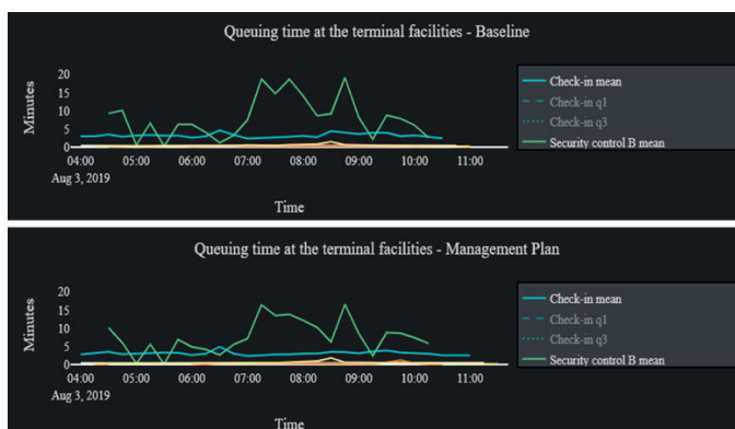
Figure 11: Queueing time in baseline and management plan for delayed departures at PMI.
