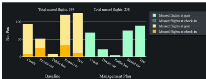
Figure 10: Missed flights in baseline and management plan for delayed departures at PMI.
