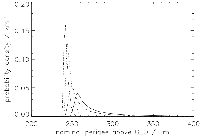
Fig. 4. Distributions of nominal perigee heights above geostationary derived for the satellite parameter distributions of Figure 1 (and disposal reliability p = 0.9 , fractional fuel measurement uncertainty \sigma_0 = 0.4 ). The parameter distribution cases are “bright & light” (solid line), “bright & heavy” (dashed line), “dark & light” (dotted line), “dark & heavy” (dash-dot line).
