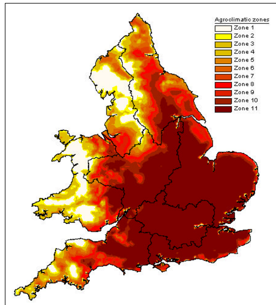
Figure 5-10. Agroclimatic zone map for UKCIP02 2050s High scenario
