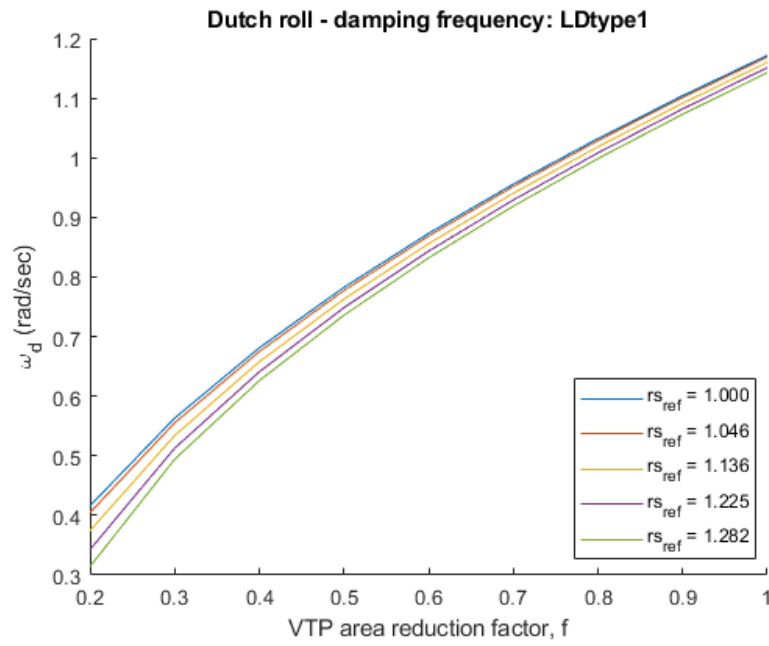
Fig. 14 Dutch roll: damping frequency for LDtype 1
