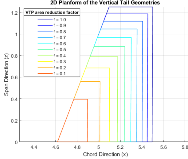
Fig. 3 Visualisation of varying VTP sizes
