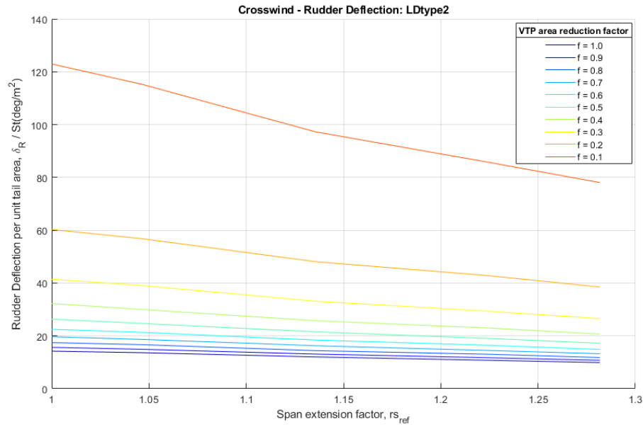
Fig. 11 Crosswind: Rudder deflection per unit area for LDtype 2
