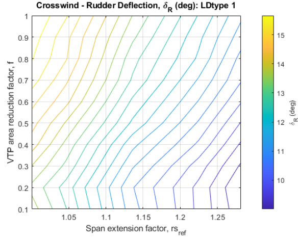
Fig. 7 Crosswind rudder deflection for LDtype 1
