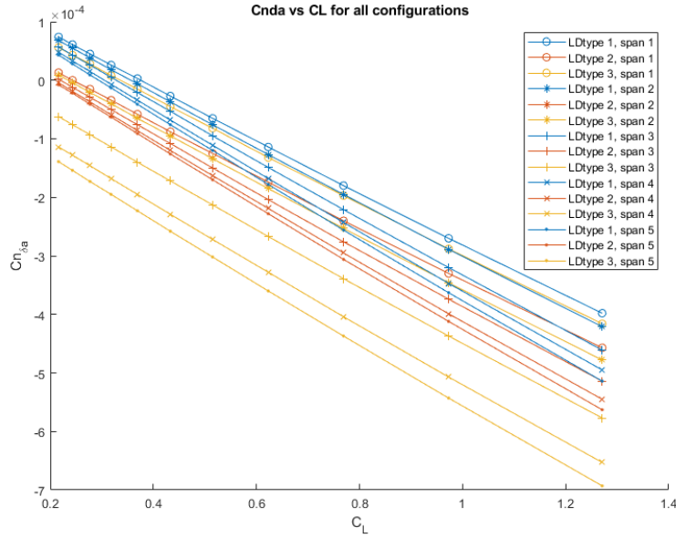
Fig. 6 Yawing moment due to aileron deflection for all configurations
