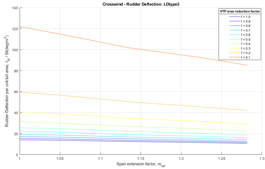
Fig. 12 Crosswind: Rudder deflection per unit area for LDtype 3
