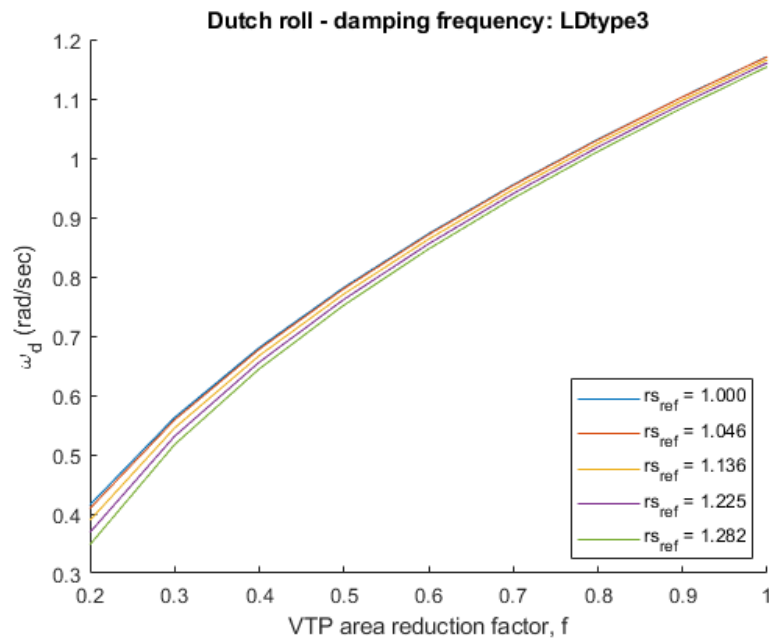
Fig. 16 Dutch roll: damping frequency for LDtype 3
