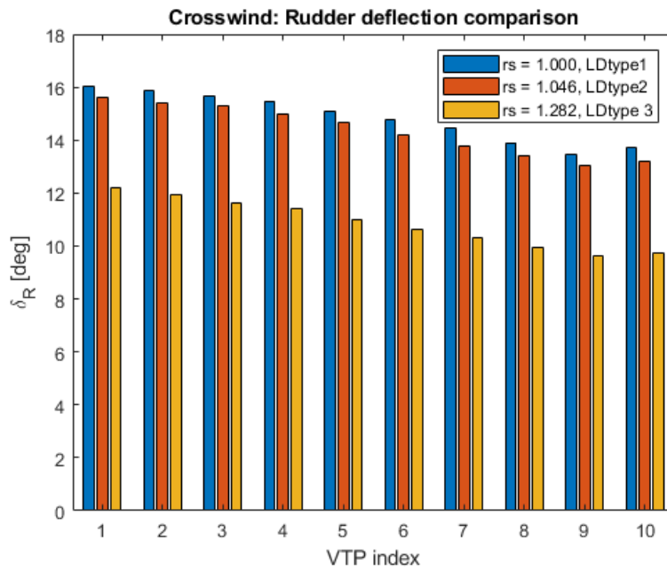
Fig. 13 Crosswind: Comparison of ideal cases
