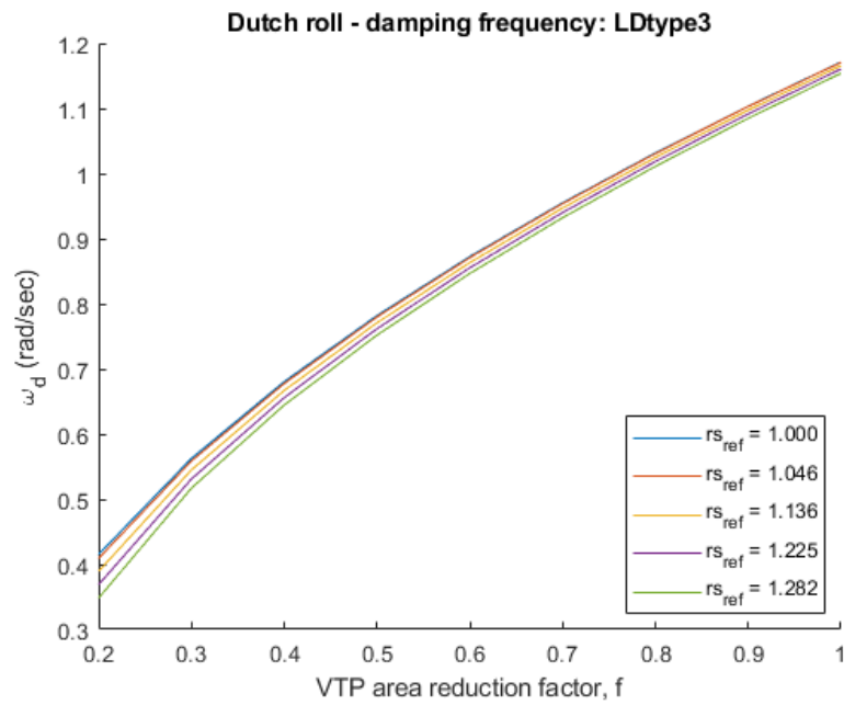
Fig. 20 Dutch roll: damping ratio for LDtype 3
