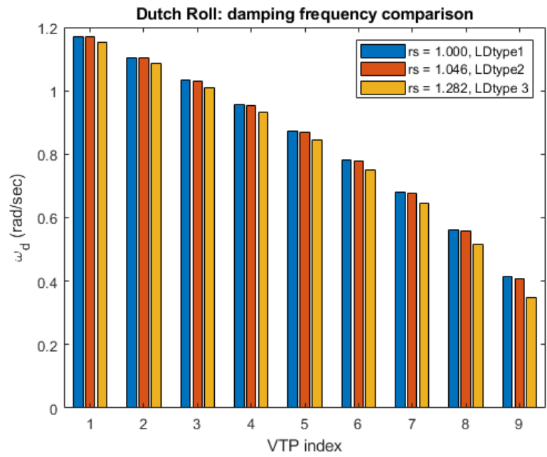
Fig. 17 Dutch roll: comparison of ideal cases - damping frequency
