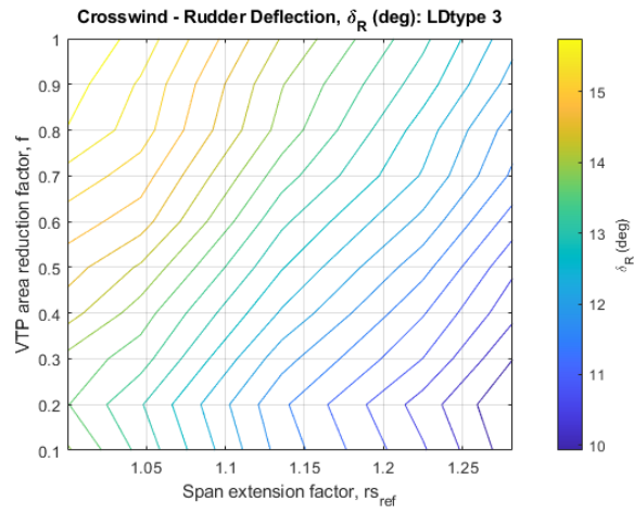
Fig. 9 Crosswind rudder deflection for LDtype 3
