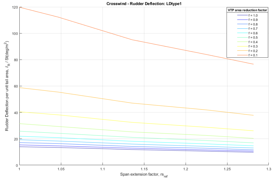
Fig. 10 Crosswind: Rudder deflection per unit area for LDtype 1
