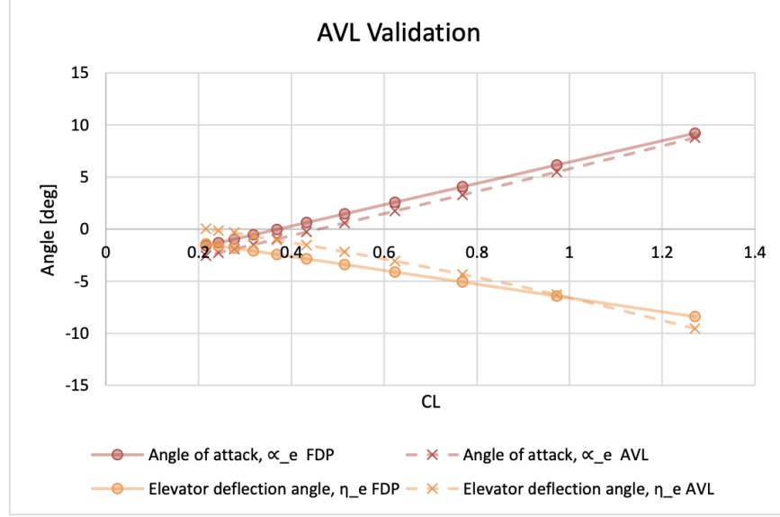
Fig. 4 AVL validation methodology
