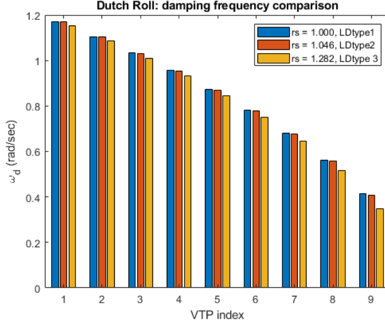
Fig. 21 Dutch roll: comparison of ideal cases - damping ratio
