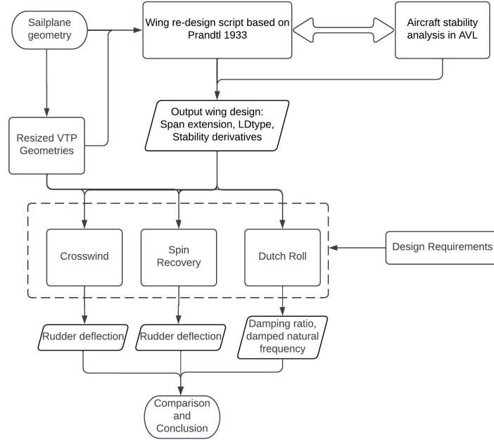
Fig. 2 Methodology flowchart
