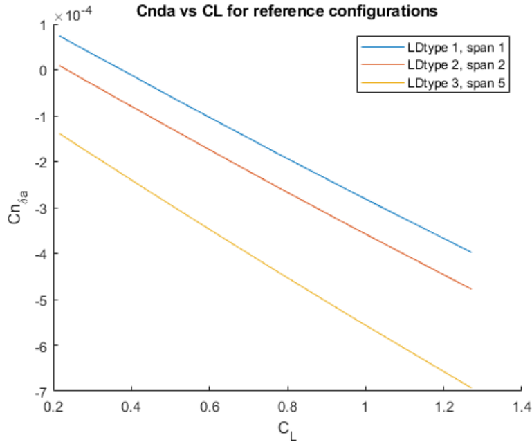
Fig. 5 Yawing moment due to aileron deflection for ideal cases
