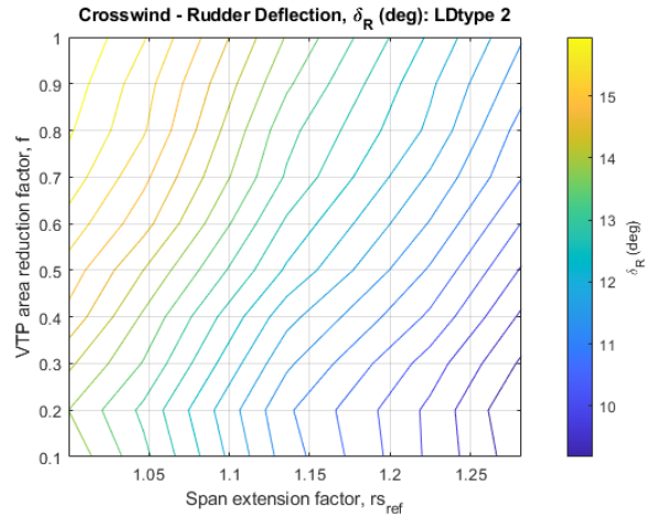
Fig. 8 Crosswind rudder deflection for LDtype 2
