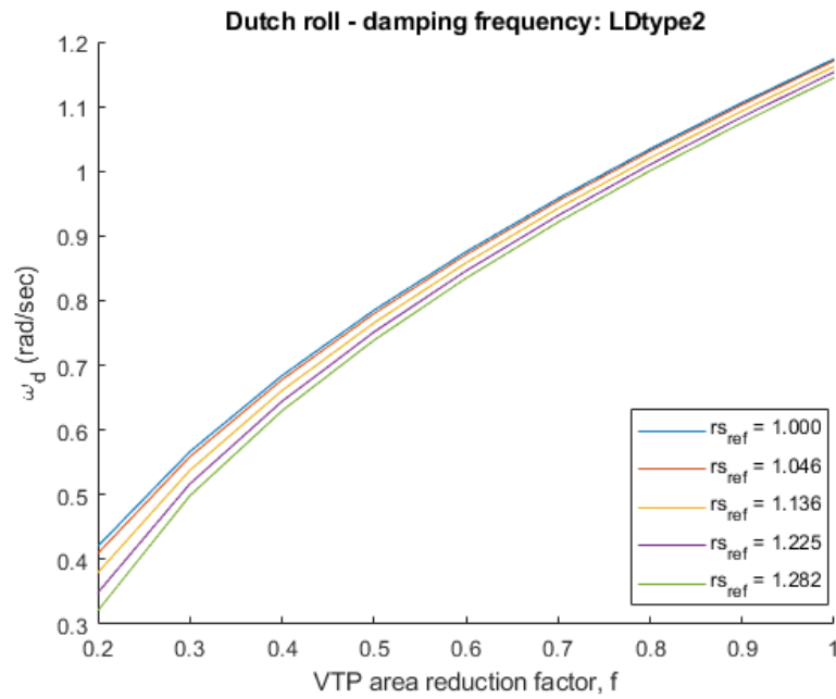
Fig. 15 Dutch roll: damping frequency for LDtype 2
