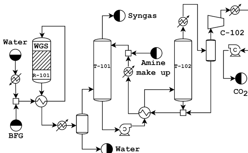
Figure 1. MDEA CO 2 capture unit (Reproduced from ref [23]. Available under a CC-BY 4.0 license. Copyright Elsevier, Khallaghi et al.[23])
