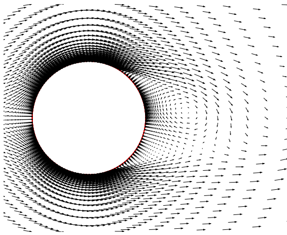
(a) Velocity vectors.
