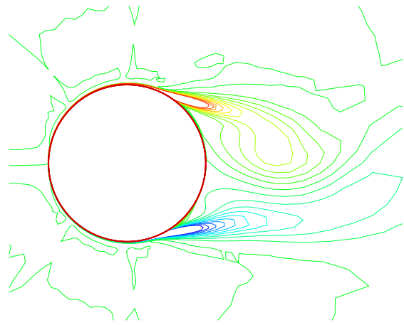
(b) Vorticity.
