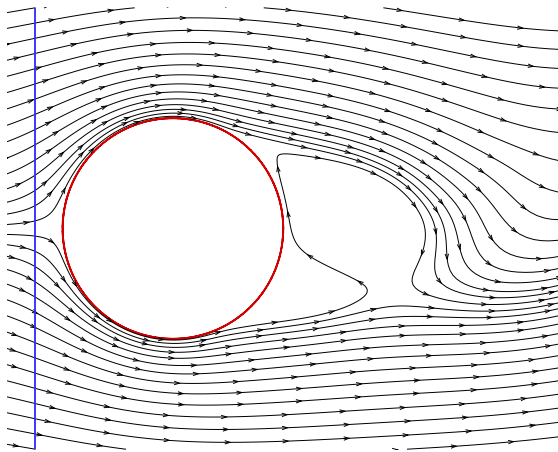
(c) Streamlines – upstream rake.
