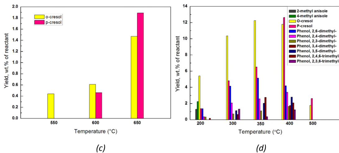
Fig. 3: Yields of main products in the liquid fraction at different temperatures in (a) non-catalytic decomposition, and (b) catalytic decomposition over HZSM-5 [HZ(25)] of anisole; and yield of methyl-phenols at different temperatures in (c) non-catalytic decomposition, and (d) catalytic decomposition over HZ(25)
