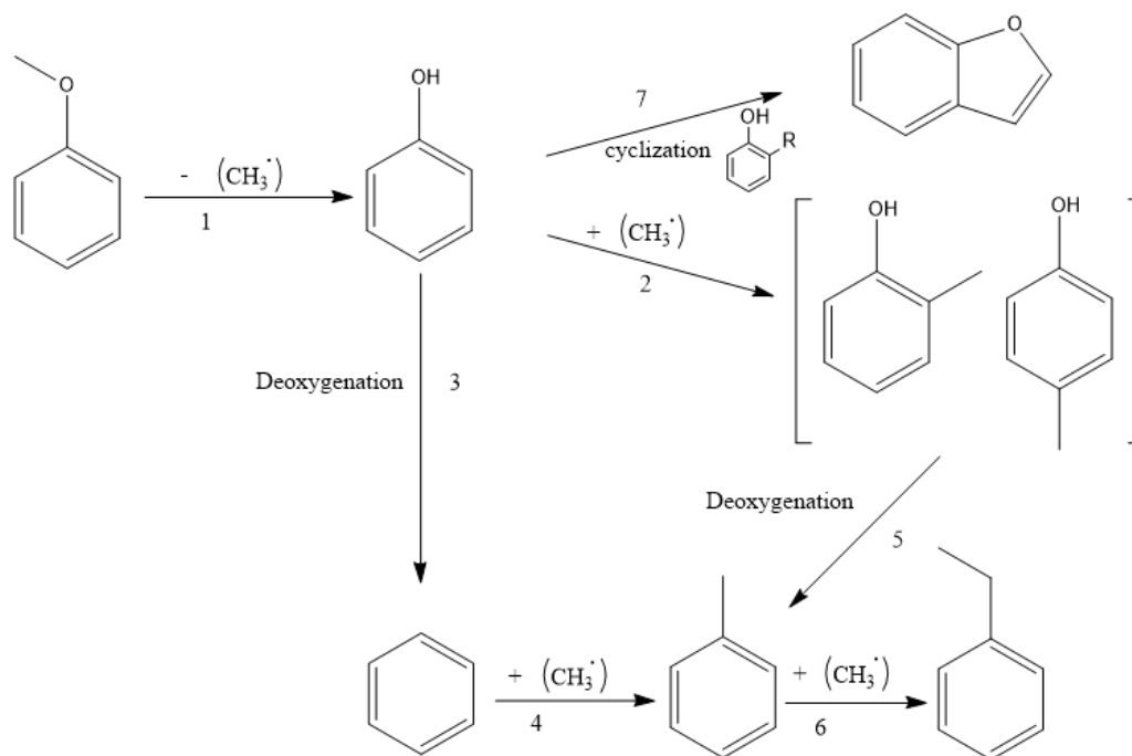
548 Fig. 6: Reaction mechanism for (a) catalytic (HZSM-5), and (b) non-catalytic transmethylation of anisole 549 decomposition
