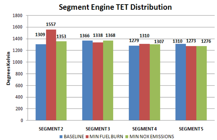
Fig. 5 Engine TET distribution among mission profile climb segments for the baseline and the optimal trajectories
