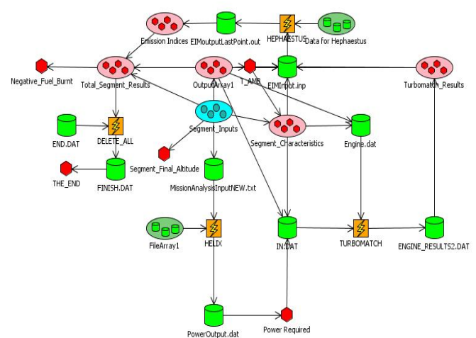
Fig. 2 Segment workflow illustration in LMS OPTIMUS
