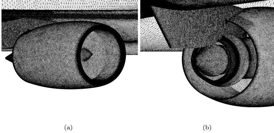
Figure 3: Close-up of the surface mesh of the installed aero-engine showing (a) the fanface, intake spinner and the nacelle, and (b) the exhaust systems and the pylon in perspective view.
