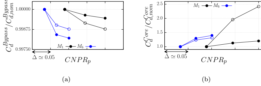
Figure 16: Variation of (a) the C_d^{Bypass}/C_{d,nom}^{Bypass} with CNPR_p , and (b) the C_d^{Core}/C_{d,nom}^{Core} with CNPR_p for the installed configuration (●) and isolated engine with the pylon (○) at constant FNPR_p .
