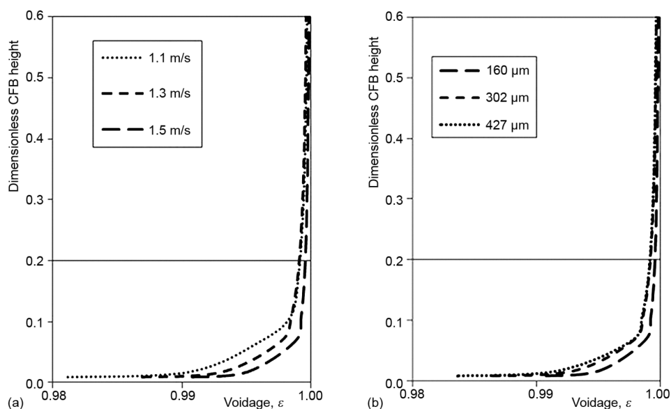
Figure 3. (a) Effect of superficial gas velocity on axial voidage profile ( d_p = 160 \mu\text{m} ), (b) effect of particle size on axial voidage profile at lower gas velocity
