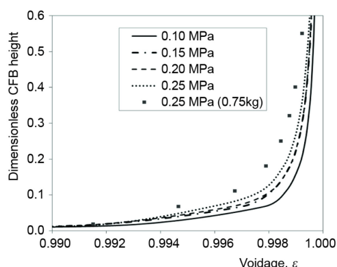
Figure 8. Voidage profile along the height for the fixed particle size ( d_p = 302 \mu\text{m} , gas velocity is 2.1 m/s, solids loading is 0.5 kg)
