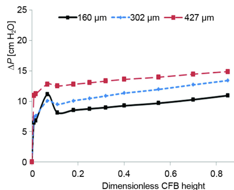
Figure 6. Effect of mean particle size on pressure drop at superficial gas velocity of 50% of U_t and bed pressure is 0.20 MPa
