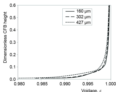
Figure 9. Effect of mean particle size on axial voidage (gas velocity 50% of U_t , bed pressure is 0.20 MPa, solids loading is 0.5 kg)
