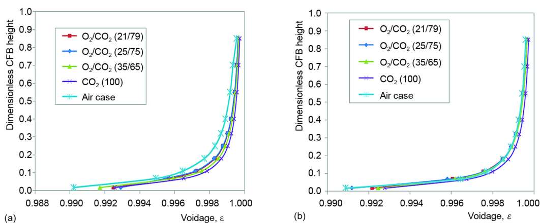
Figure 4. (a) Bed voidage vs. O_2/CO_2 mixture (gas velocity is 1.1 m/s, solids loading is 0.5 kg), (b) bed voidage vs. O_2/CO_2 mixture (gas velocity is 1.5 m/s, solids loading is 0.5 kg)
