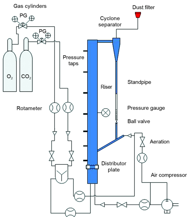
Figure 1. The CFB riser (air and O 2 /CO 2 mode)
