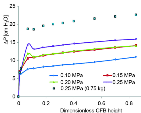
Figure 5. Effect of operating pressure on pressure drop at gas velocity 2.1 m/s ( d_p = 302 \mu\text{m} , solids loading is 0.5 kg)
