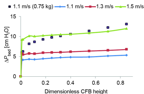
Figure 2. Effect of superficial gas velocity on \Delta P_{\text{bed}} over the bed ( d_p = 160 \mu\text{m} , solids loading is 0.5 kg)
