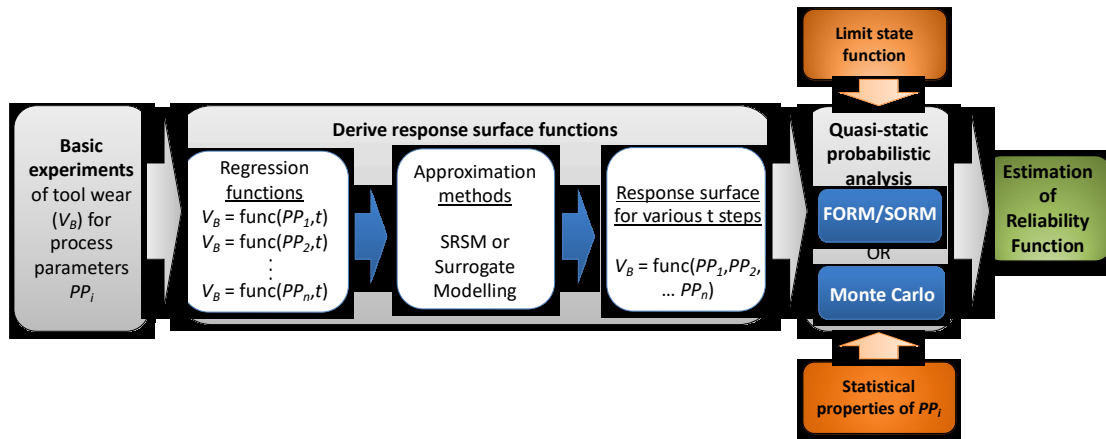
Figure 5: The proposed methodology to assess cutting tool reliability based on cutting forces
