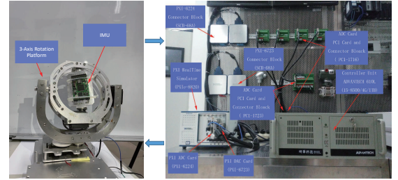
Fig. 3: System test platform
