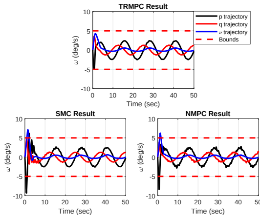
Fig. 6: Angular rate evolution trajectories
